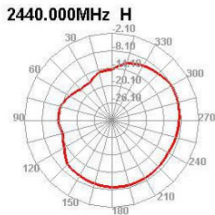
Figure 2-7 Antenna pattern Peak gain: -1dBi; average gain: -3dBi
