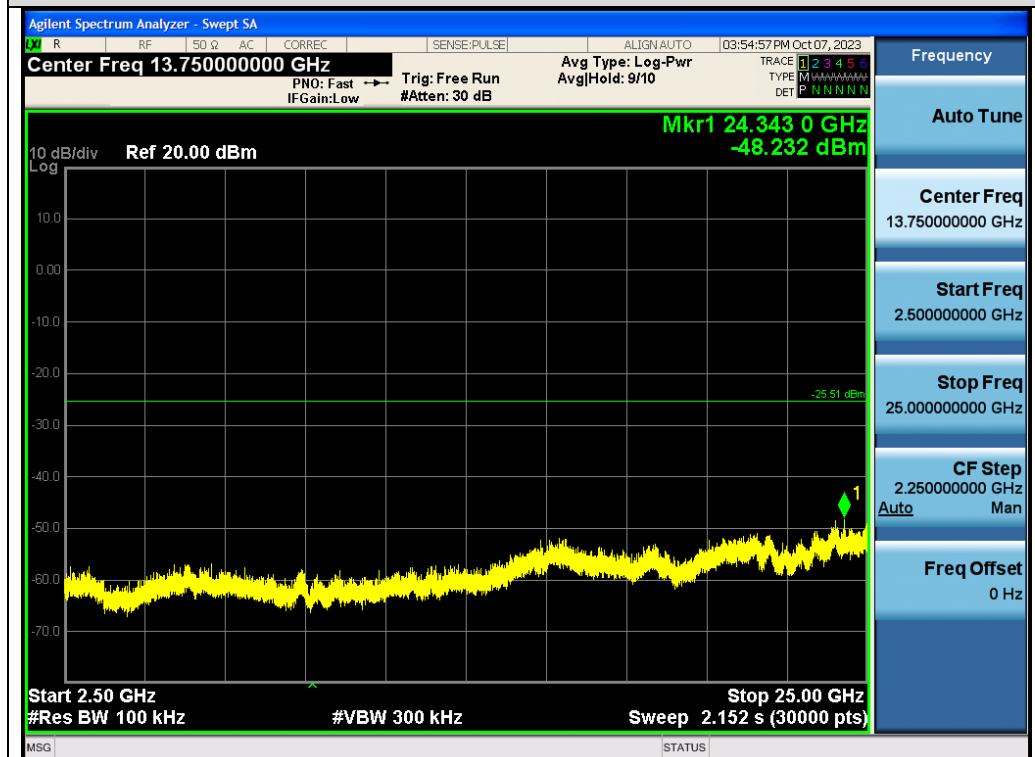
Test Graph EDR ANT1 2480 2Mbps Higher Band Emissions
