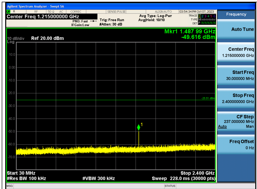
Test Graph EDR ANT1 2480 2Mbps Lower Band Emissions
