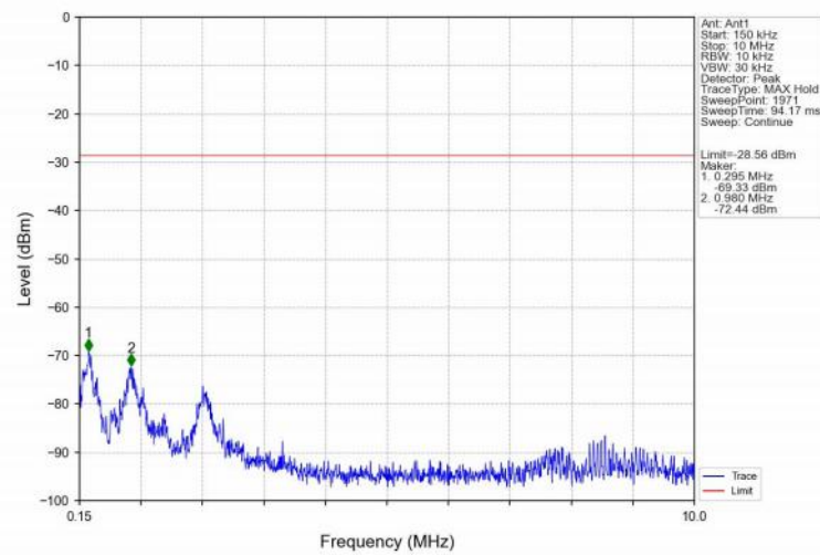
GFSK_DH5_LCH_2402MHz_Ant1_NTNV
