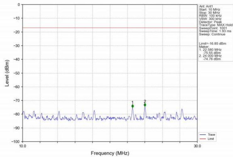
8DPSK_3DH5_MCH_2441MHz_Ant1_NTNV
