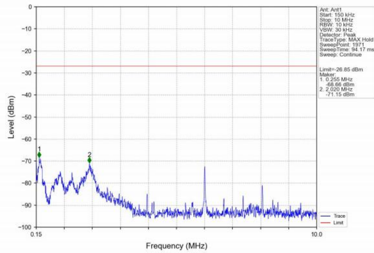
8DPSK_3DH5_MCH_2441MHz_Ant1_NTNV
