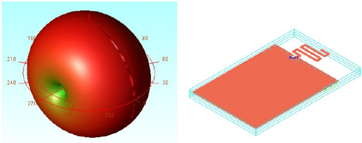
Figure 9. 3-D radiation pattern overview
