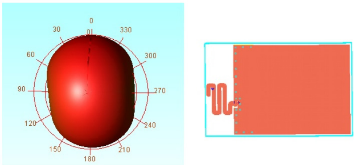
Figure 10. Radiation pattern on X-Z plane
