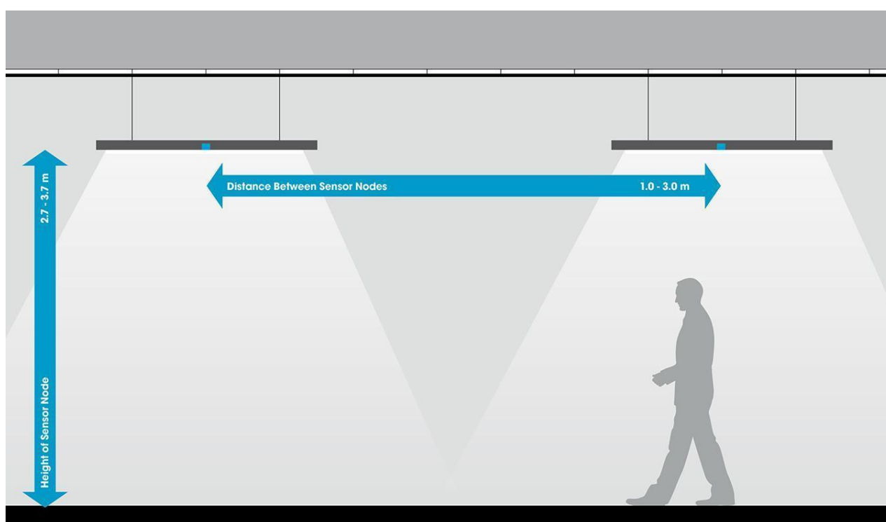
Figure 3: Recommended mounting height and neighbour spacing.
