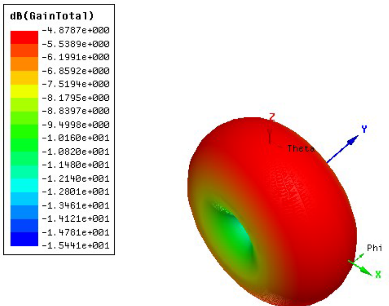
Figure 3 Gain
