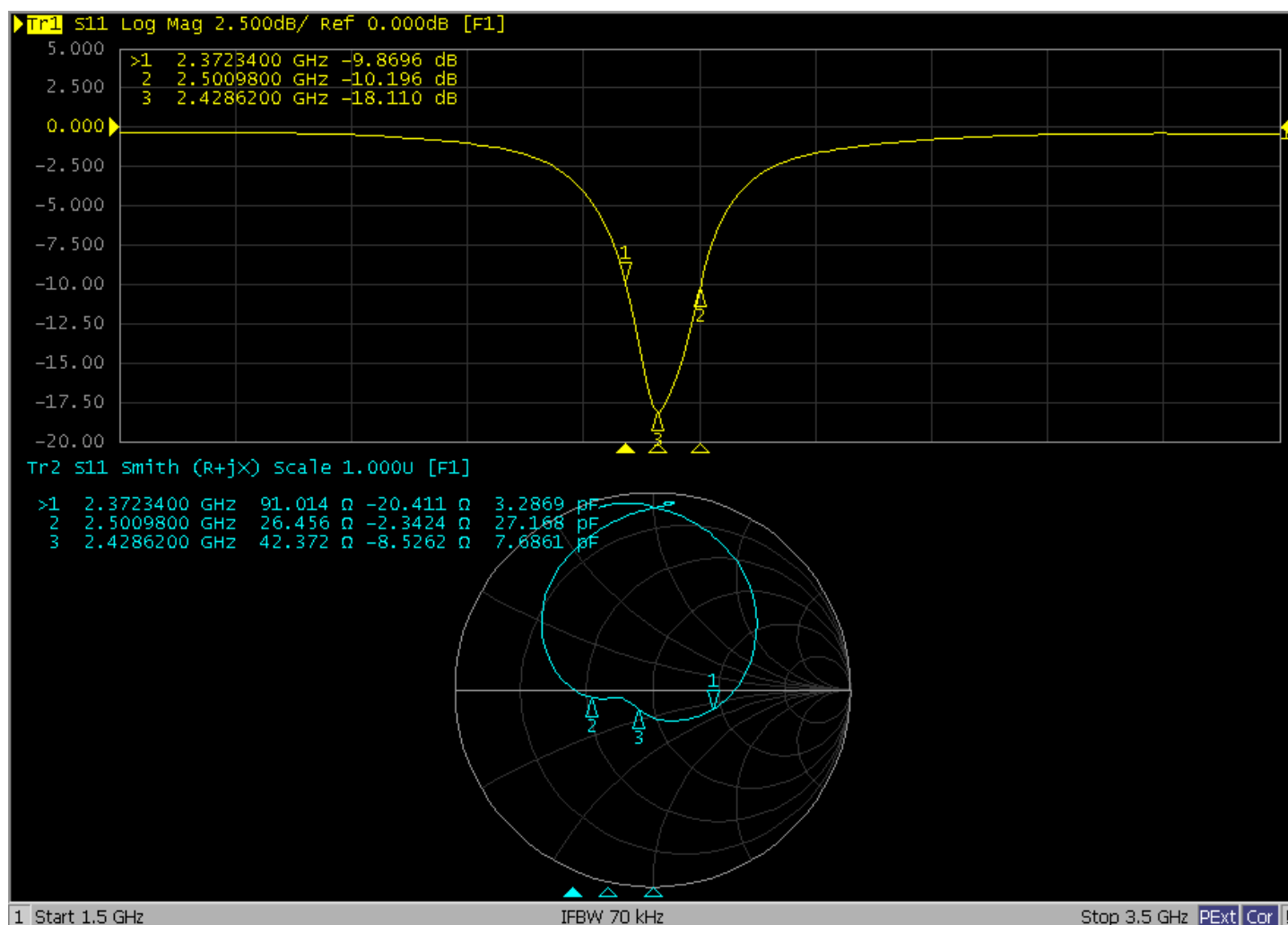
Figure 1 S11
