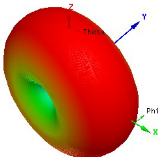
Figure 3 Gain
