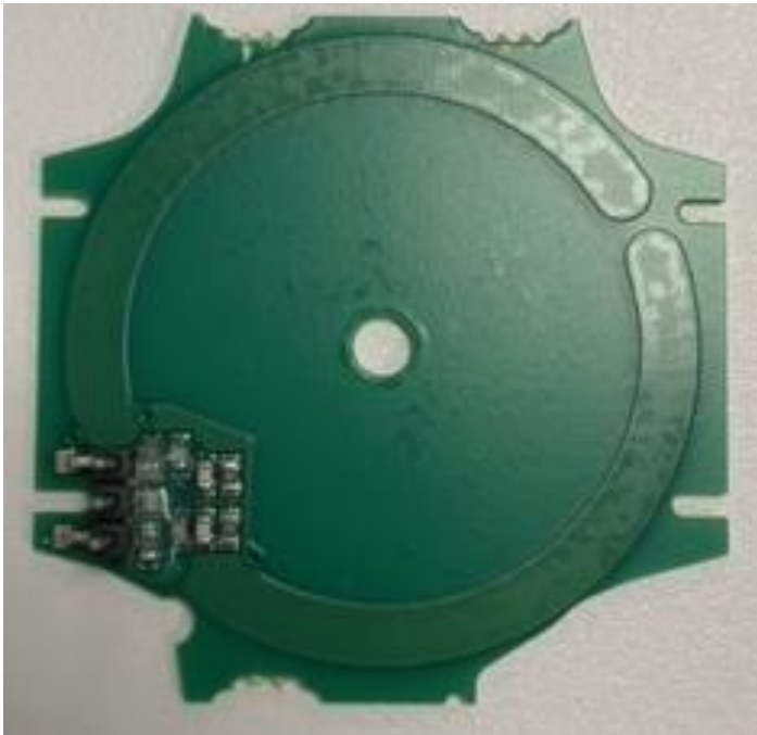
Component side of the antenna board
