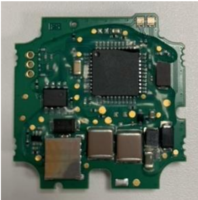
Solder side with metal shield
