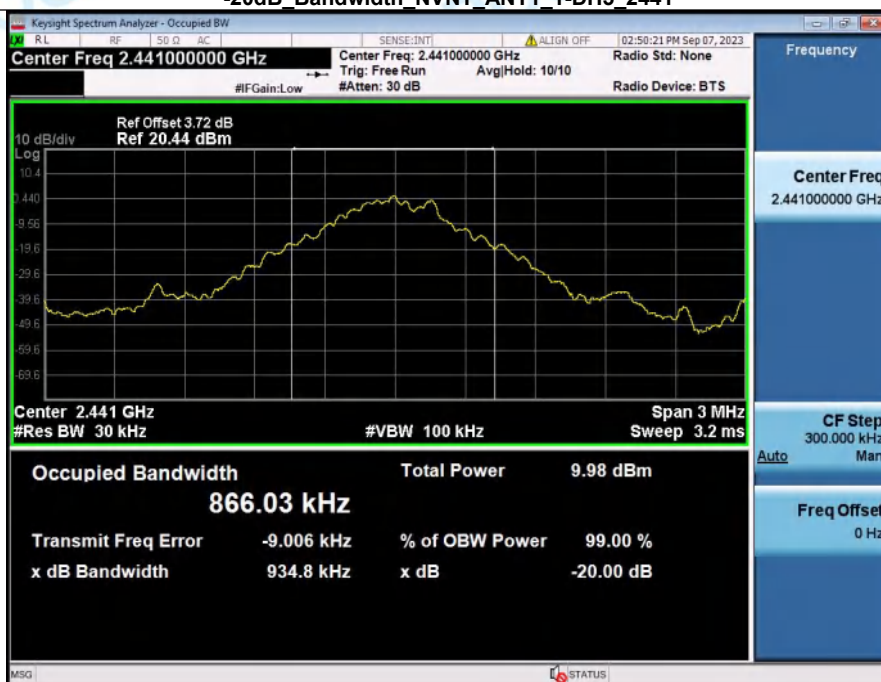
-20dB_Bandwidth_NVNT_ANT1_1-DH5_2441
