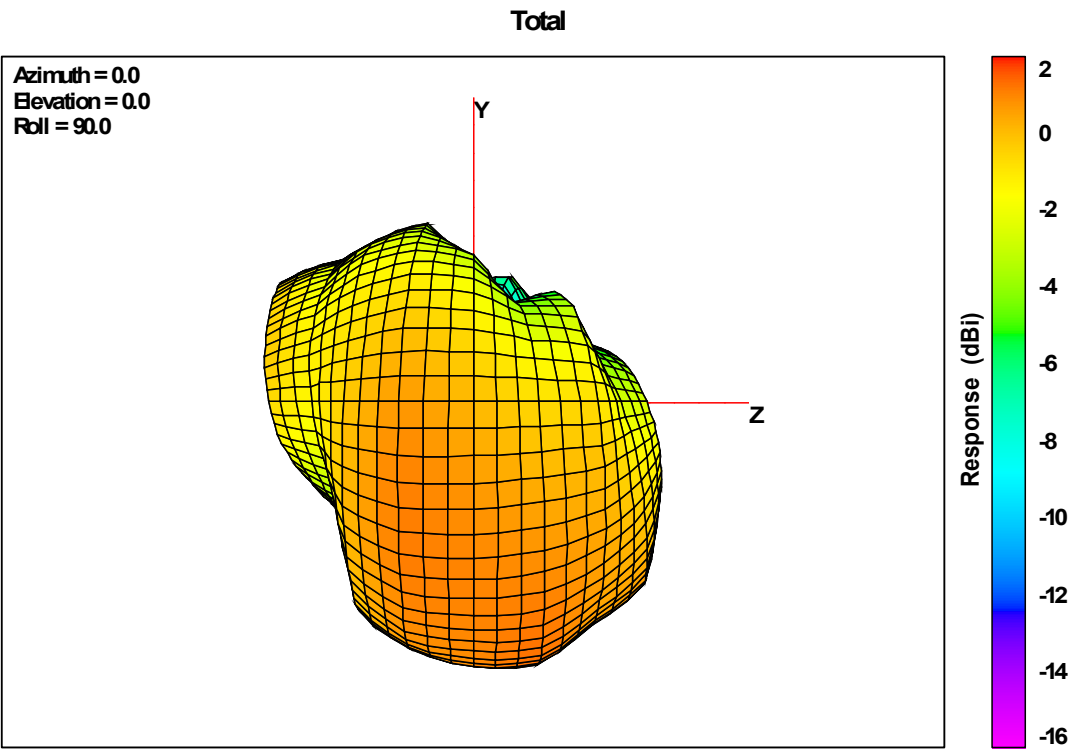
Side View 2450MHz
