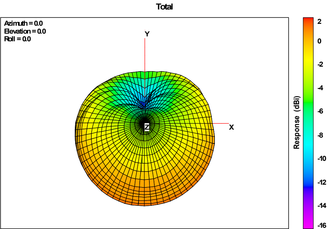
Front View 2450MHz
