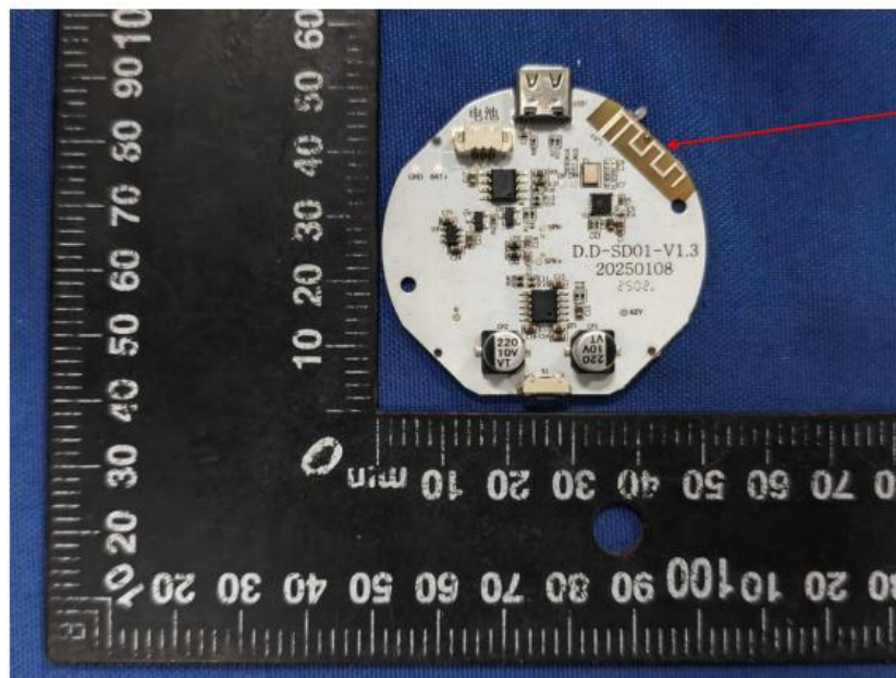
BT Antenna
