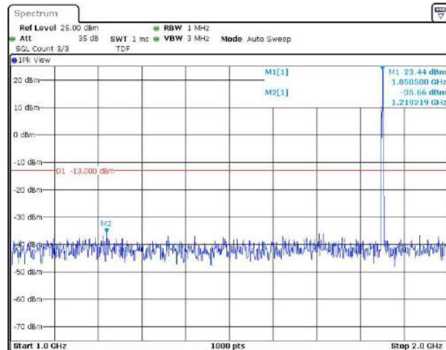
Band2-1.4MHz-QPSK-18607-1RB#0-Range2:1000~2000MHz
