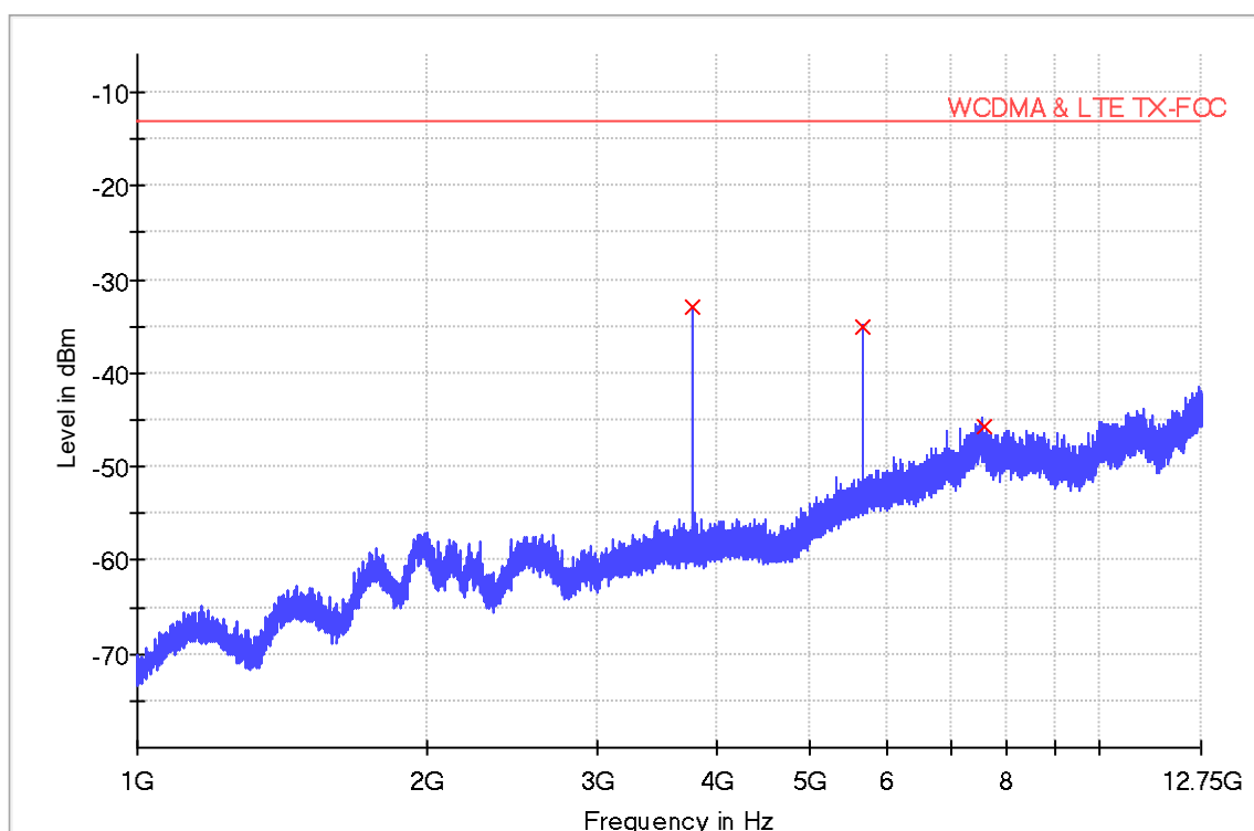
WCDMA &amp; LTE TX 1-12.75G dBm
