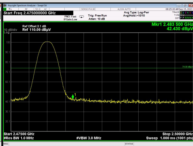
Peak Value(Horizontal)
