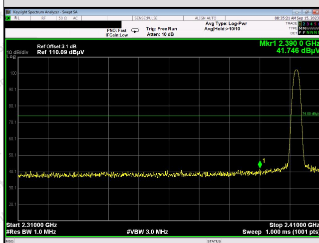
Peak Value(Vertical)
