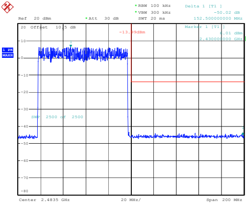
3DH1_Hopping_Upper
