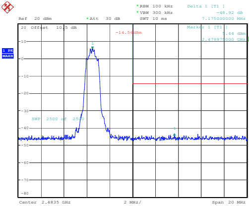
3DH1_High
