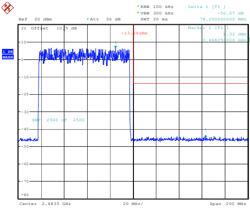
2DH1_Hopping_Upper
