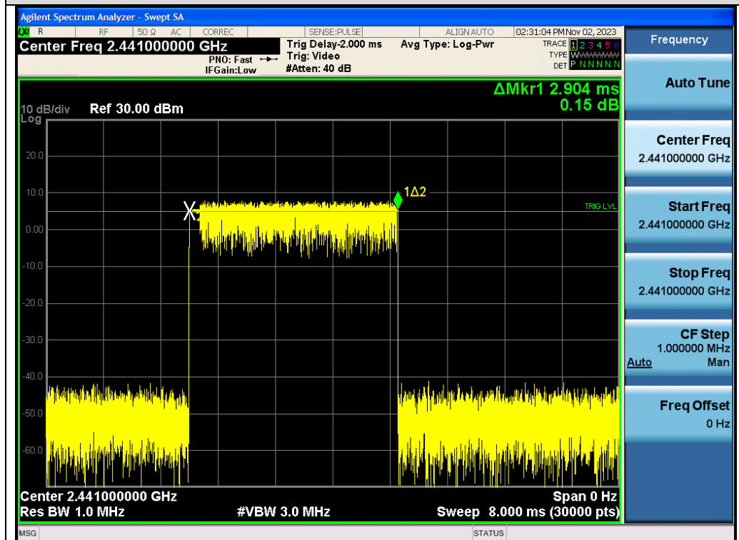
Test Graph EDR HOP ANT1 NA 3Mbps 2441 Time per Burst
