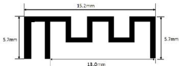
Antenna Photo & Length (mm)
