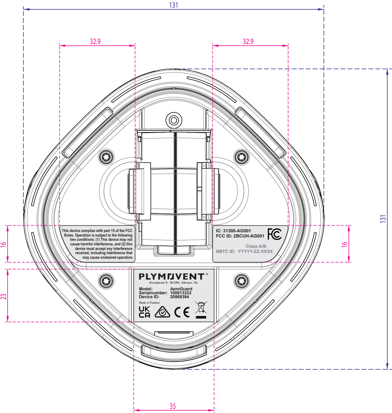
Bottom side with lid removed (all dimensions in mm)
