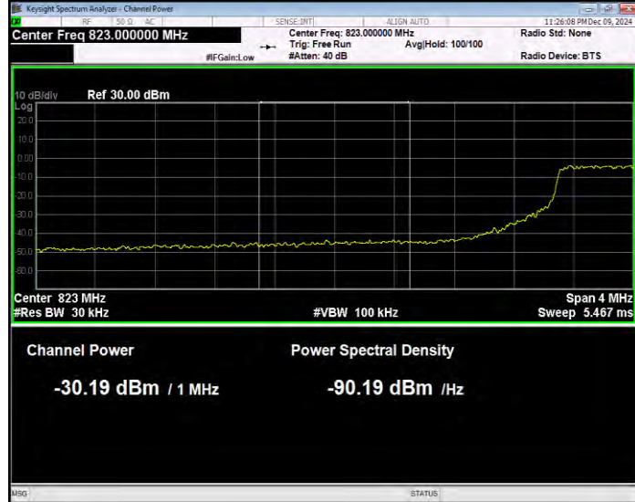
Band26(824-849) 16QAM BW=10MHz Channel=26840 RB Size=1 Position=#Max Extended
