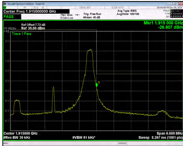
Band25 16QAM BW=3MHz Channel=26675 RB Size=15 Position=#0 Extended
