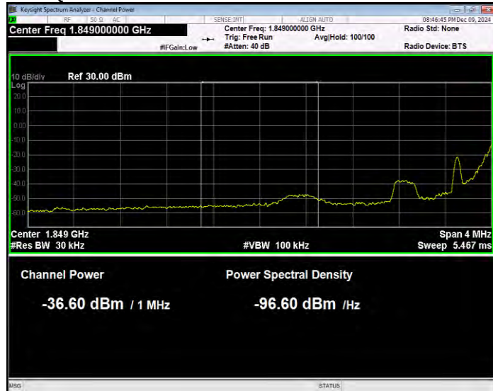
Band25 16QAM BW=1.4MHz Channel=26047 RB Size=1 Position=#0 Extended
