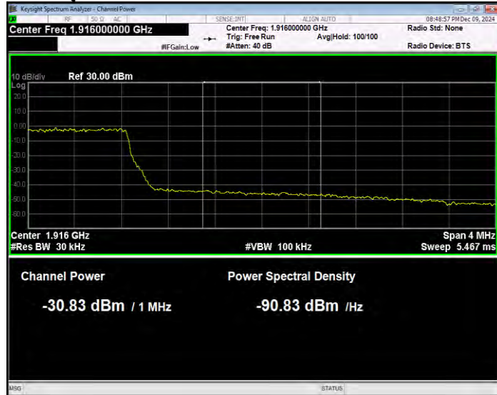
Band25 16QAM BW=3MHz Channel=26675 RB Size=1 Position=#Max Extended
