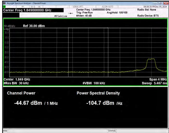
Band25 QPSK BW=10MHz Channel=26090 RB Size=1 Position=#0 Extended
