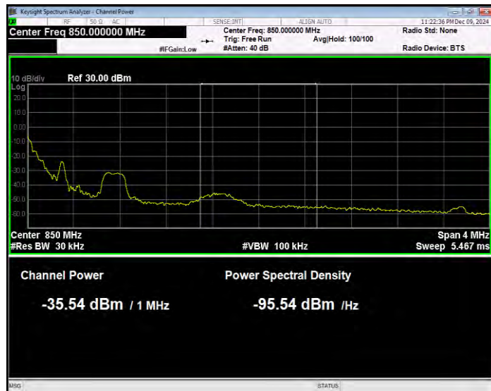
Band26(824-849) 16QAM BW=1.4MHz Channel=26797 RB Size=6 Position=#0 Extended
