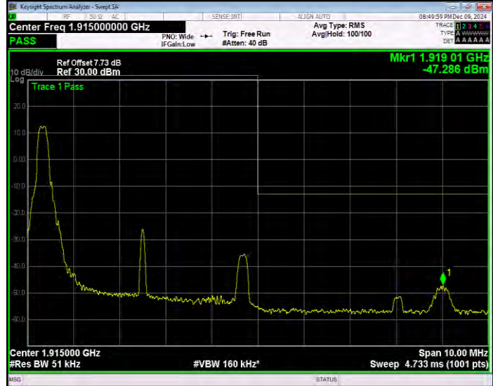
Band25 16QAM BW=5MHz Channel=26665 RB Size=1 Position=#Max Extended
