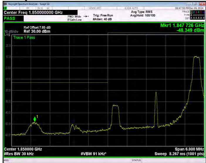
Band25 QPSK BW=3MHz Channel=26055 RB Size=15 Position=#0 Extended
