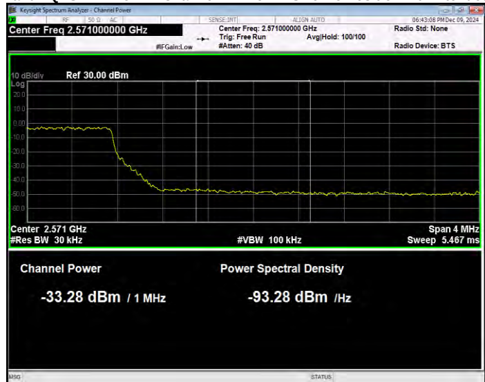
Band7 QPSK BW=5MHz Channel=21425 RB Size=25 Position=#0 Normal
