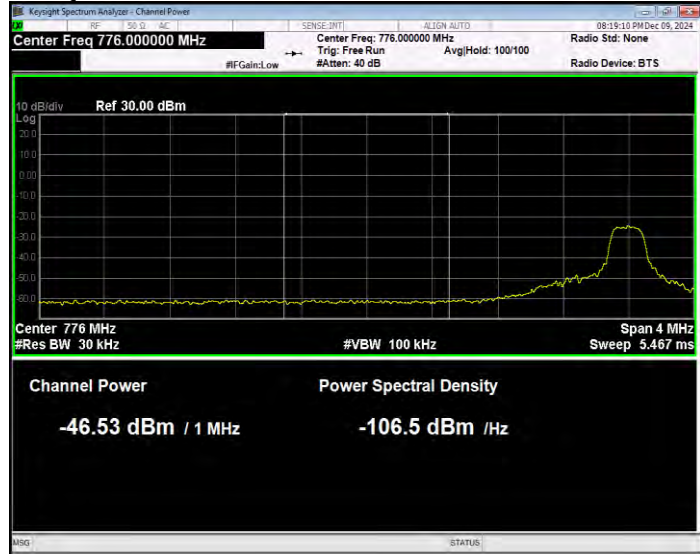
Band13 QPSK BW=10MHz Channel=23230 RB Size=1 Position=#Max Normal
