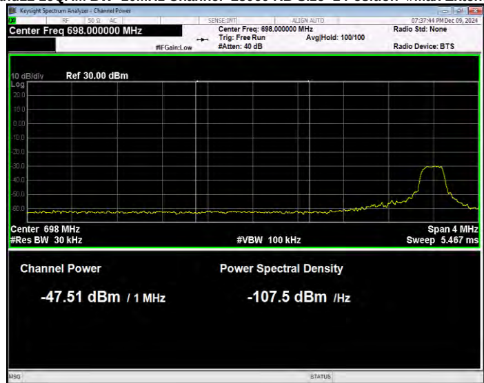
Band12 16QAM BW=10MHz Channel=23060 RB Size=1 Position=#0 Extended
