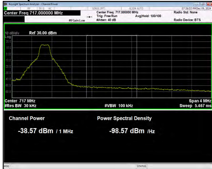
Band12 16QAM BW=5MHz Channel=23155 RB Size=1 Position=#0 Extended
