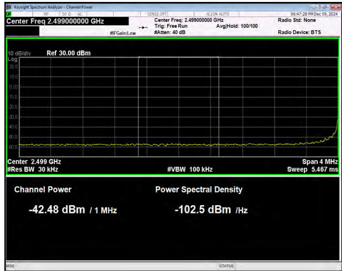
Band7 16QAM BW=20MHz Channel=20850 RB Size=100 Position=#0 Extended
