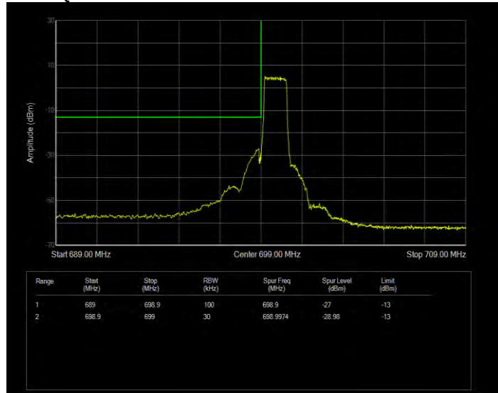
Band12 QPSK BW=10MHz Channel=23060 RB Size=1 Position=#0 Extended
