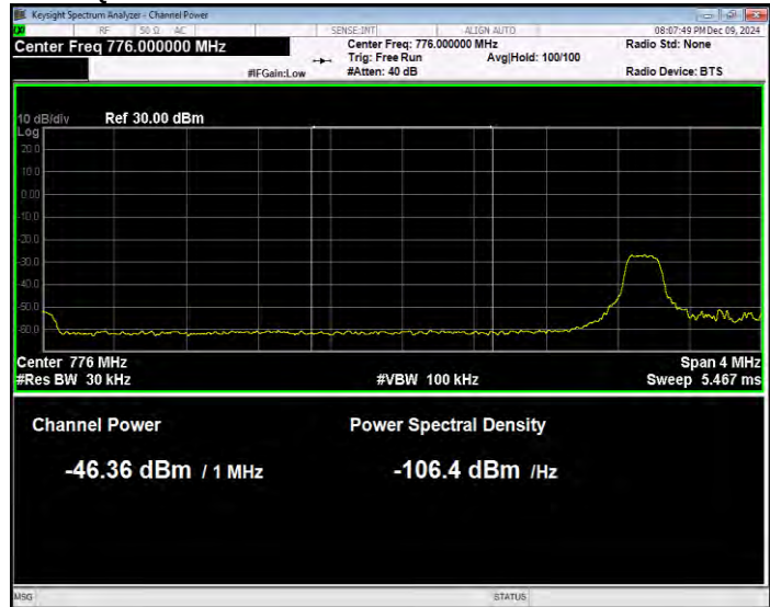
Band13 16QAM BW=5MHz Channel=23205 RB Size=1 Position=#Max Normal
