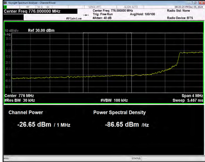
Band13 QPSK BW=10MHz Channel=23230 RB Size=1 Position=#Max Extended
