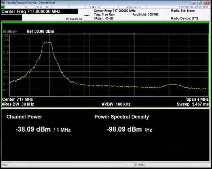
Band12 QPSK BW=3MHz Channel=23165 RB Size=1 Position=#0 Extended
