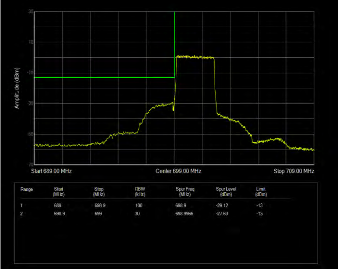
Band12 QPSK BW=3MHz Channel=23025 RB Size=1 Position=#0 Extended
