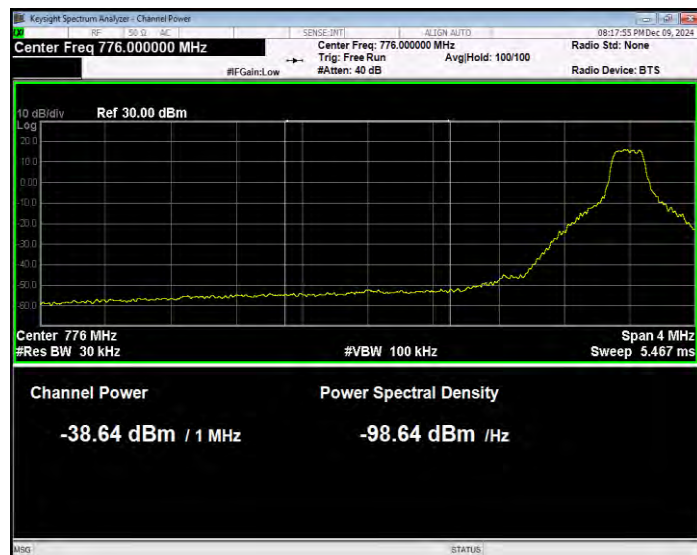
Band13 QPSK BW=10MHz Channel=23230 RB Size=1 Position=#0 Normal
