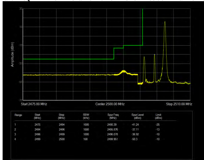
Band7 16QAM BW=5MHz Channel=21425 RB Size=1 Position=#0 Extended
