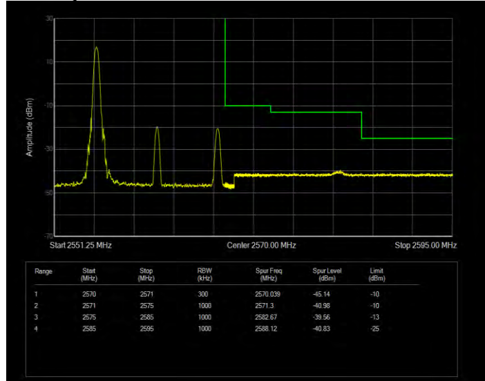
Band7 16QAM BW=15MHz Channel=21375 RB Size=1 Position=#Max Normal
