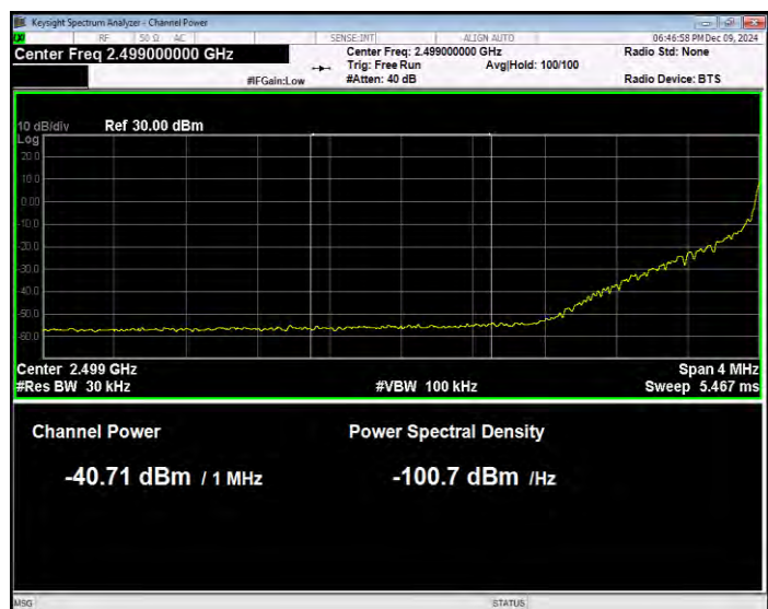
Band7 QPSK BW=20MHz Channel=20850 RB Size=1 Position=#0 Normal
