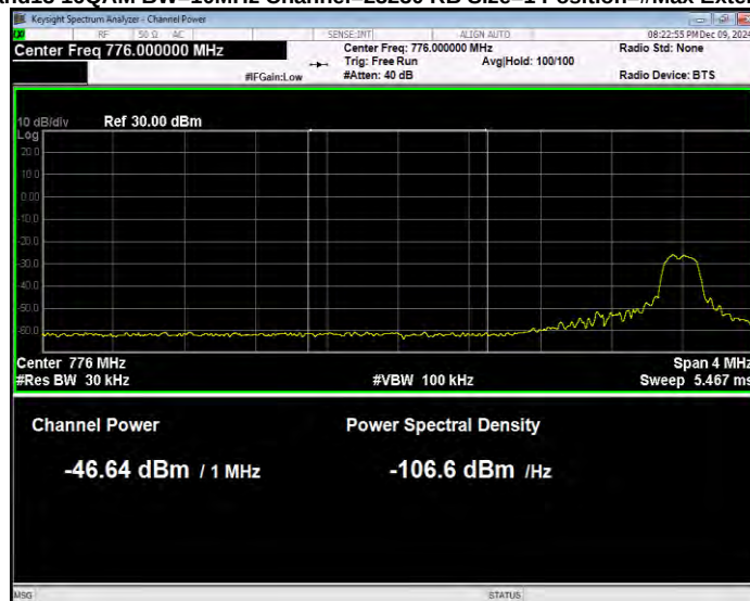
Band13 16QAM BW=10MHz Channel=23230 RB Size=1 Position=#0 Extended
