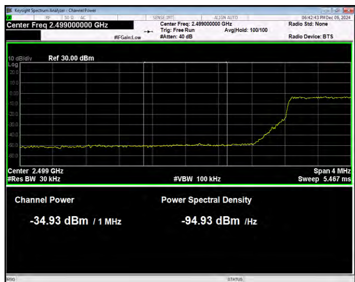
Band7 16QAM BW=5MHz Channel=20775 RB Size=1 Position=#Max Normal
