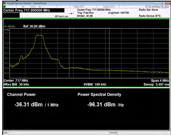
Band12 QPSK BW=1.4MHz Channel=23173 RB Size=1 Position=#0 Extended
