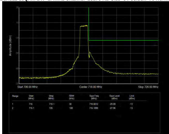
Band12 16QAM BW=10MHz Channel=23130 RB Size=1 Position=#0 Extended
