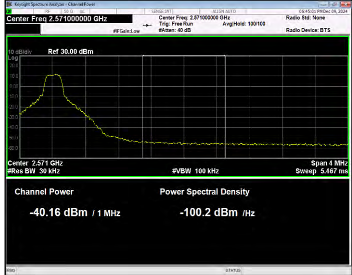
Band7 16QAM BW=10MHz Channel=21400 RB Size=1 Position=#Max Normal
