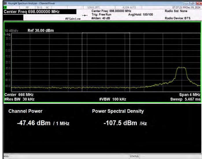
Band12 QPSK BW=10MHz Channel=23060 RB Size=1 Position=#Max Normal
