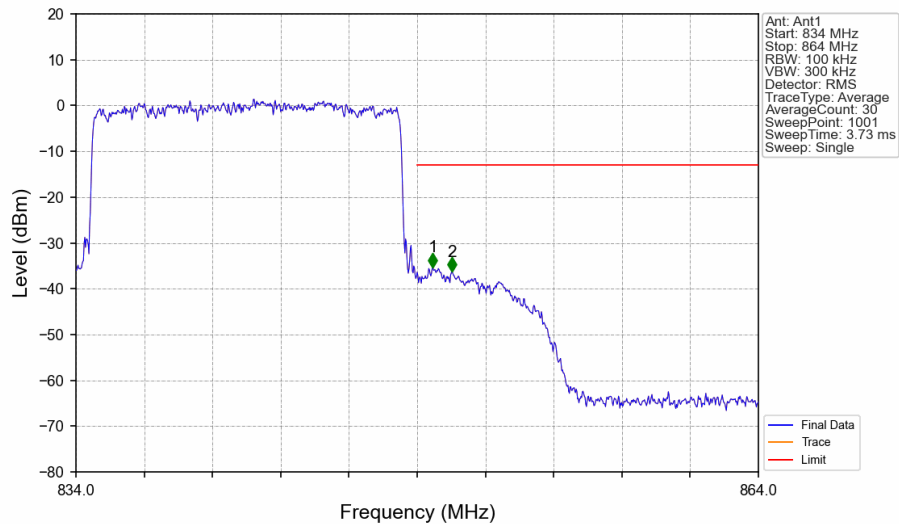
Band26b_15MHz_16QAM_HCH_841.5MHz_RB_75_0_NTNV
