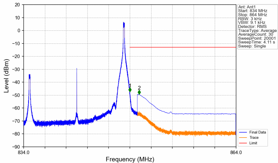
Band26b_15MHz_16QAM_HCH_841.5MHz_RB_1_74_NTNV
