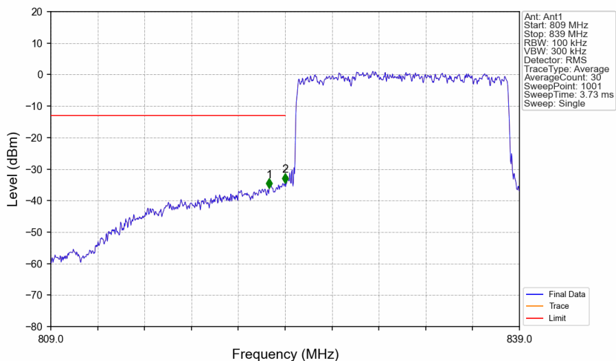
Band26b_15MHz_16QAM_LCH_831.5MHz_RB_75_0_NTNV
