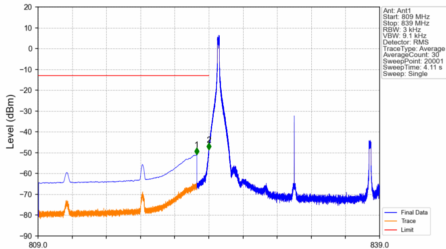
Band26b_15MHz_16QAM_LCH_831.5MHz_RB_1_0_NTNV
