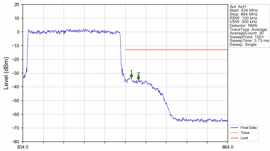
Band26b_15MHz_QPSK_HCH_841.5MHz_RB_75_0_NTNV
