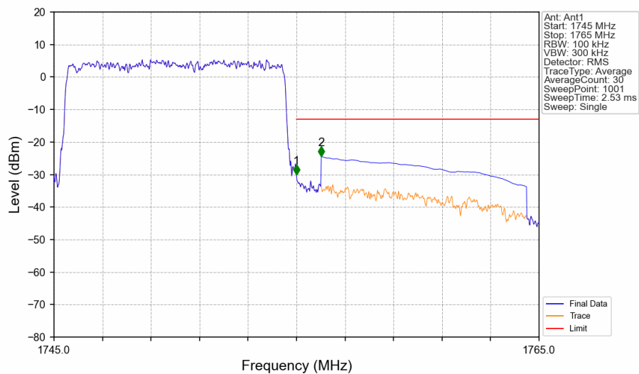
Band4_10MHz_16QAM_HCH_1750MHz_RB_50_0_NTNV
