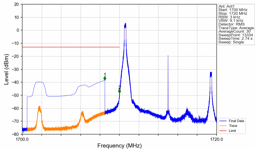
Band4_10MHz_16QAM_LCH_1715MHz_RB_1_0_NTNV
