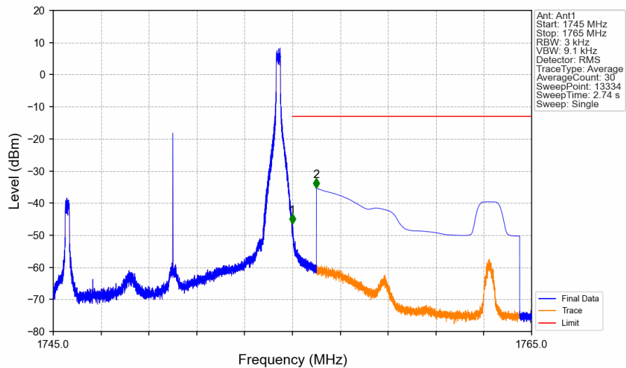
Band4_10MHz_16QAM_HCH_1750MHz_RB_1_49_NTNV
