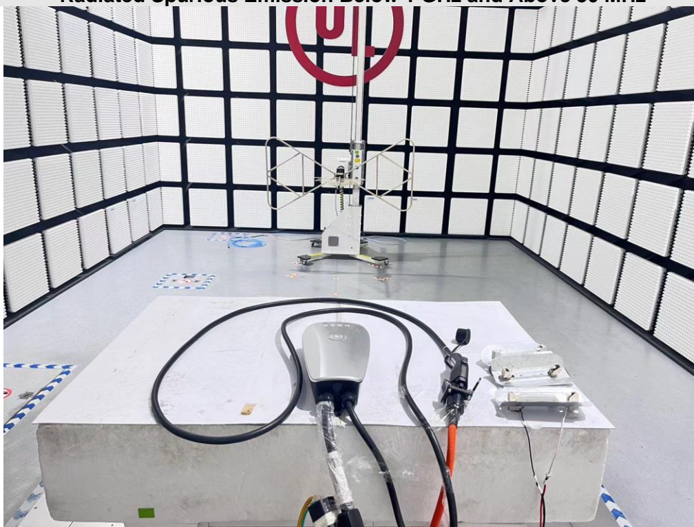
Radiated Spurious Emission Below 1 GHz and Above 30 MHz
