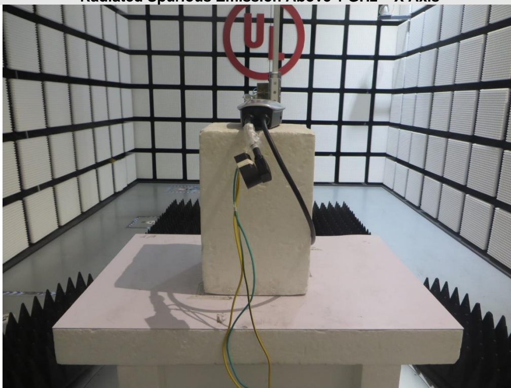
Radiated Spurious Emission Above 1 GHz – X Axis
