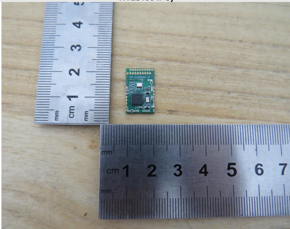
Internal View of EUT-12 (BT module-1; FCC ID: 2ADXEHY-234004PC, IC: 32291-HY234004PC)
