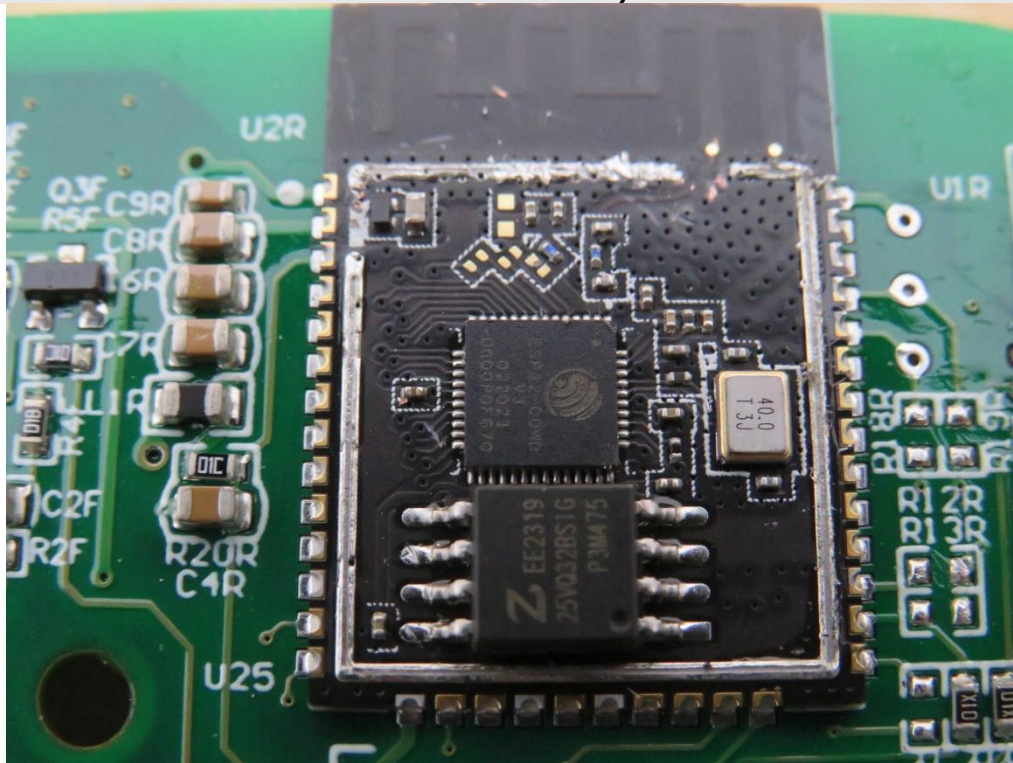
Internal View of EUT-10 (WIFI Module; FCC ID: 2AC7Z-ESP32WROOM32E, IC: 21098-ESPWROOM32E)
