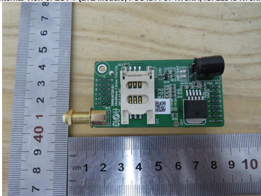
Internal View of EUT-7 (LTE module; FCC ID: PJ7-N75NA, IC: 21545-N75NA)
