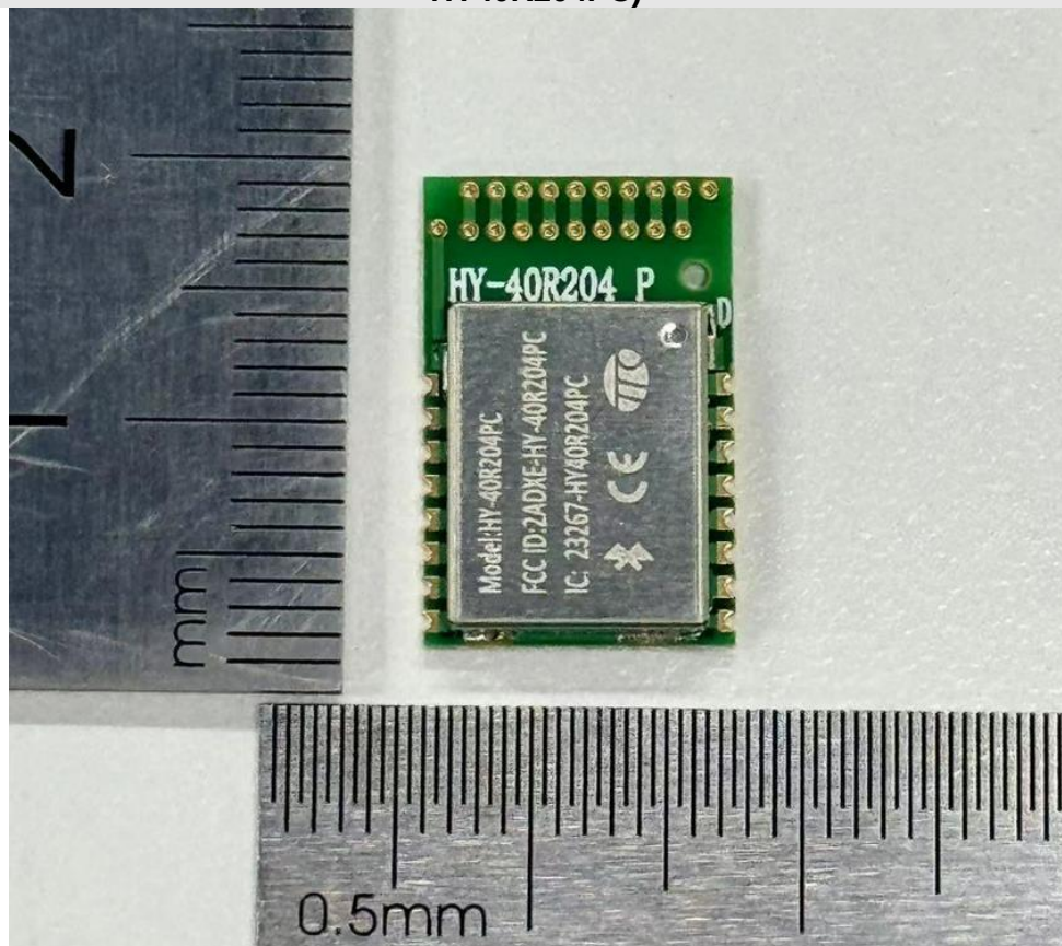
Internal View of EUT-13 (BT module-2; FCC ID: 2ADXE-HY-40R204PC, IC: 23267-HY40R204PC)
