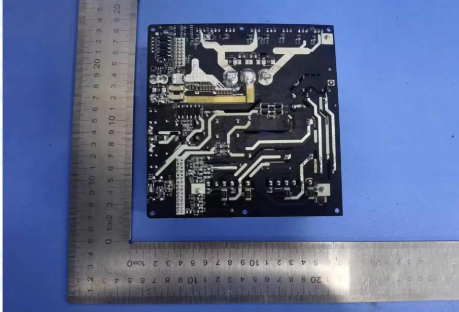
Photo 28 Appearance of PCB
