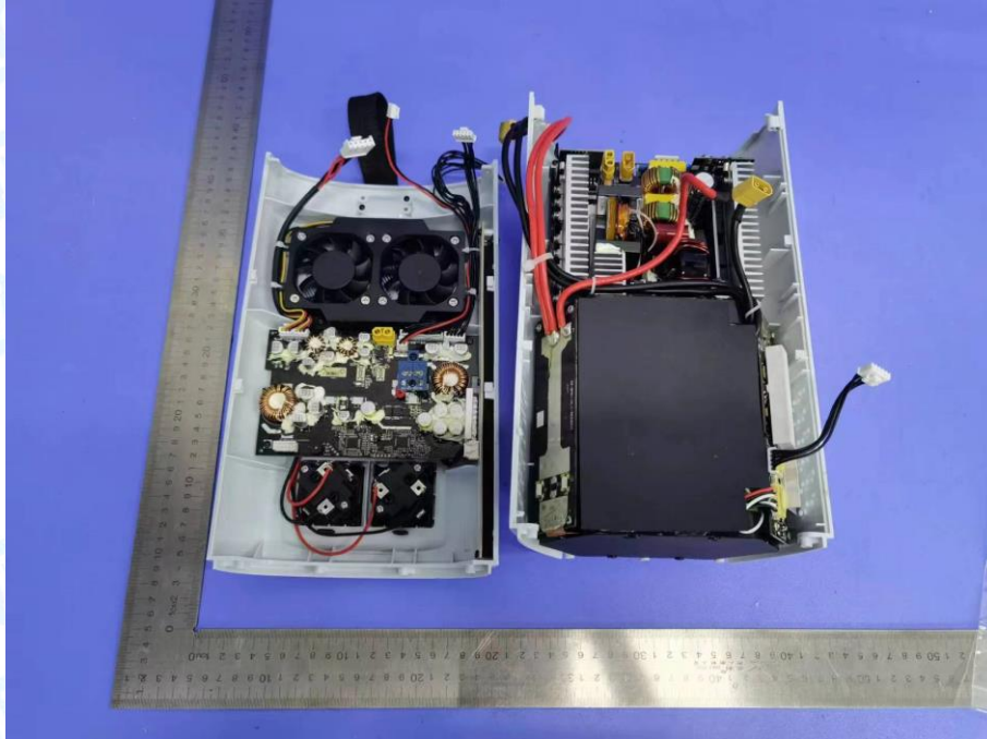
Photo 19 Internal of EUT
