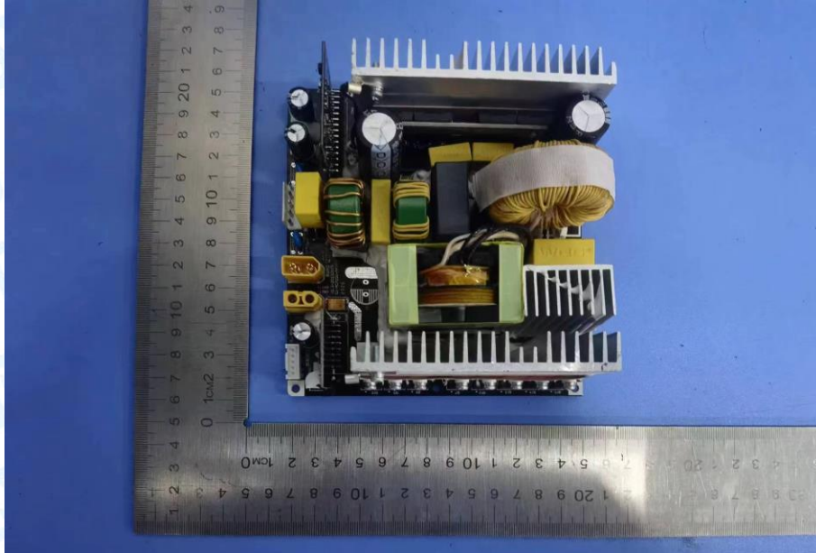
Photo 25 Appearance of PCB
