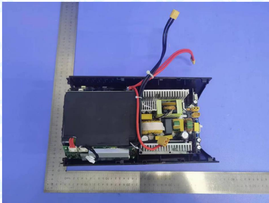
Photo 23 Internal of EUT
