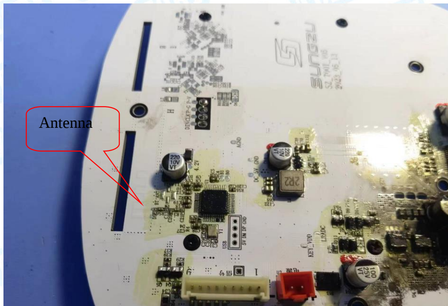
Photo 19 Internal of EUT
