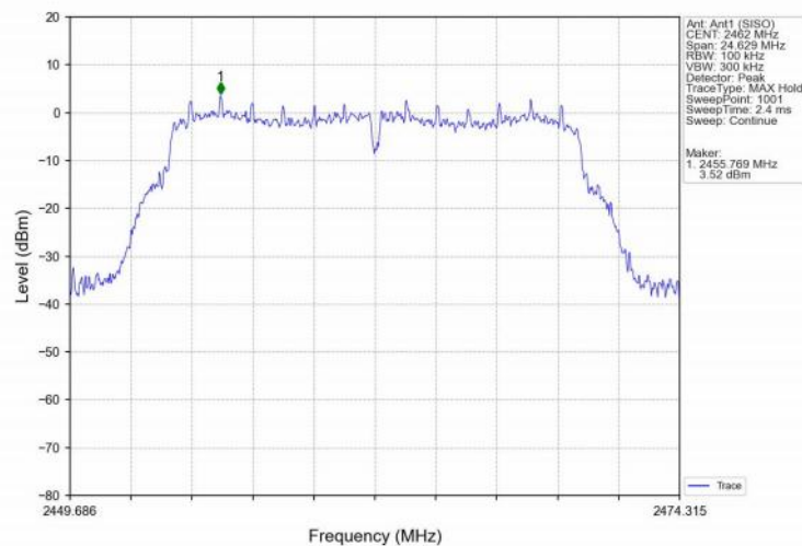
802.11g_HCH_2462MHz_Ant1 (SISO) NTN
