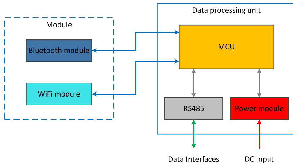
Figure 2 Overall block diagram of DAT
