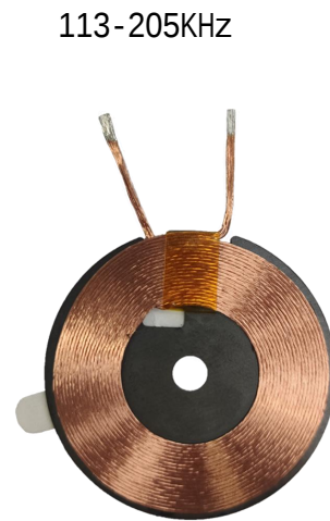
Physical drawing
