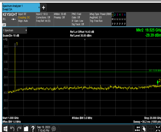
Band25-15MHz-QPSK-26115-1RB#0-Range2:1000~20000MHz
