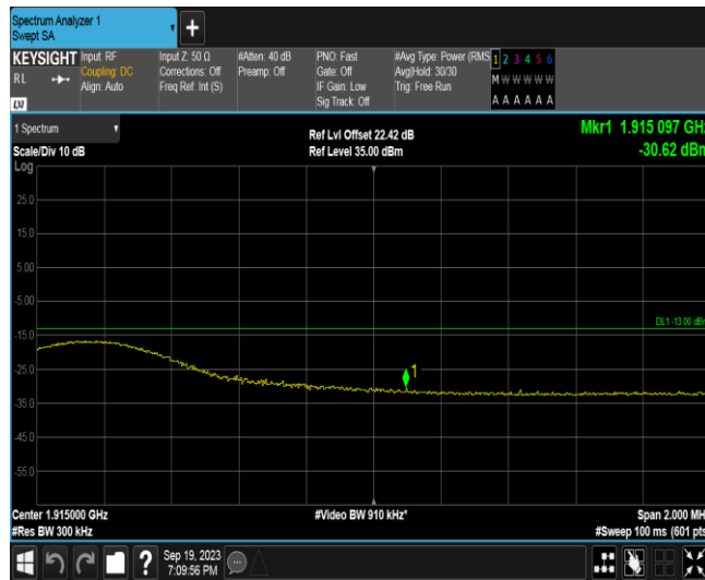
Band25-15MHz-16QAM-26615-1RB#74
