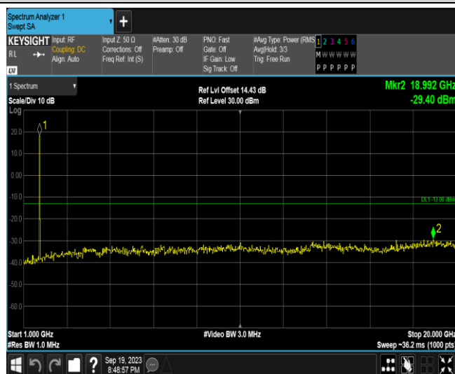
Band66-3MHz-16QAM-131987-1RB#0-Range2:1000~20000MHz
