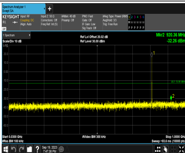
Band26B-1.4MHz-16QAM-26697-1RB#0-Range1:30~1000MHz
