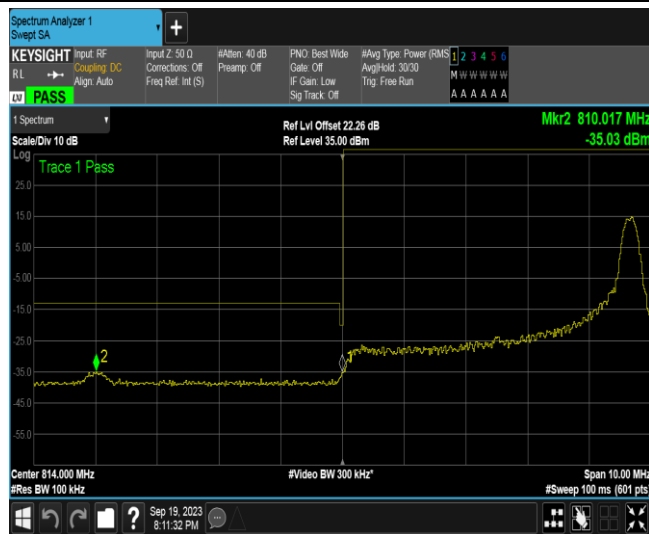
Band26B-5MHz-16QAM-26715-25RB#0
