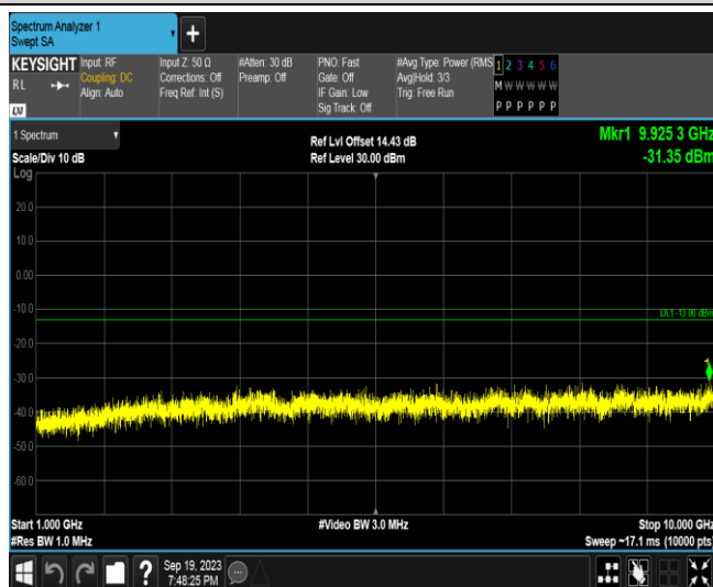
Band26B-1.4MHz-16QAM-26783-1RB#0-Range2:1000~10000MHz
