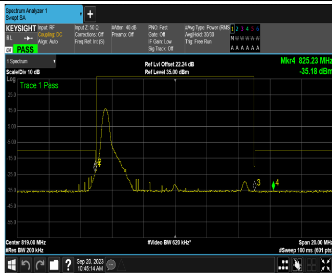
Band26B-10MHz-QPSK-26740-1RB#49
