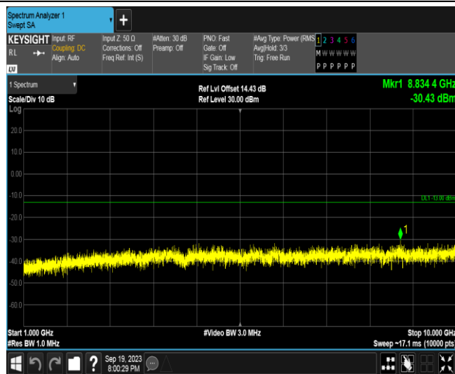
Band26B-3MHz-16QAM-26740-1RB#0-Range2:1000~10000MHz
