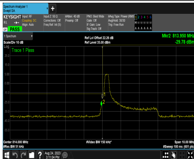
Band26B-3MHz-16QAM-26705-1RB#0
