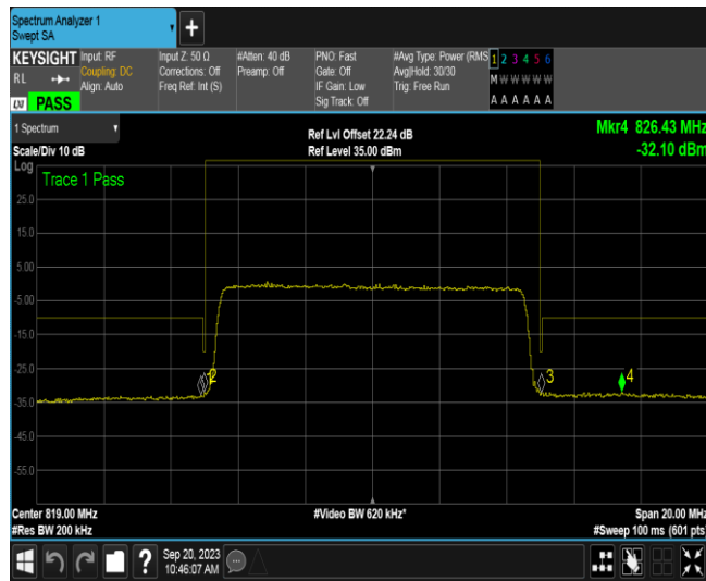
Band26B-15MHz-QPSK-26765-1RB#0
