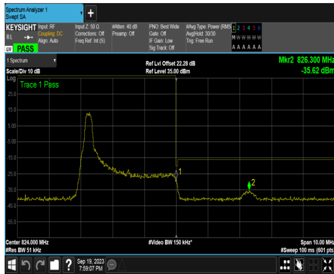
Band26B-3MHz-16QAM-26775-1RB#14
