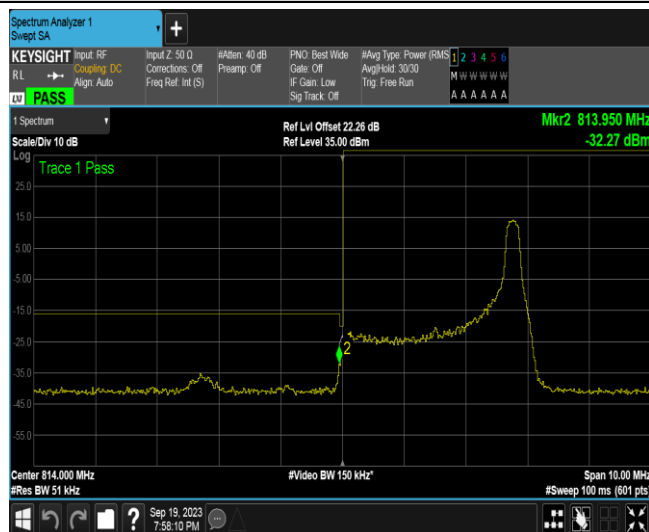
Band26B-3MHz-QPSK-26705-1RB#14
