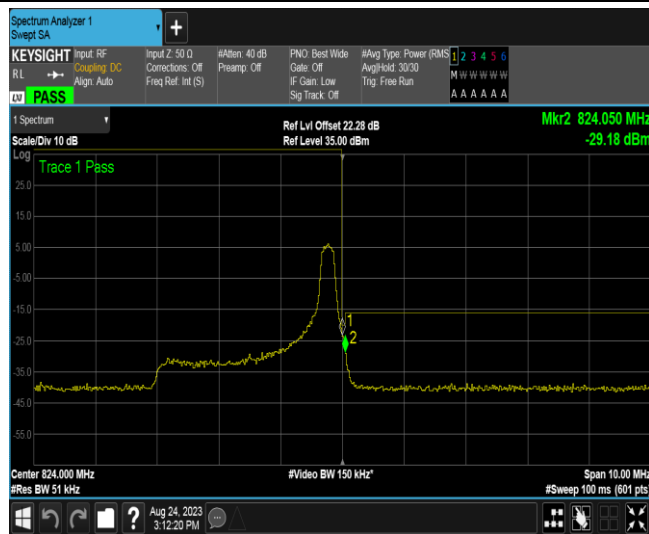
Band26B-3MHz-QPSK-26775-15RB#0
