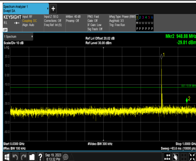
Band26B-5MHz-QPSK-26740-1RB#0-Range1:30~1000MHz
