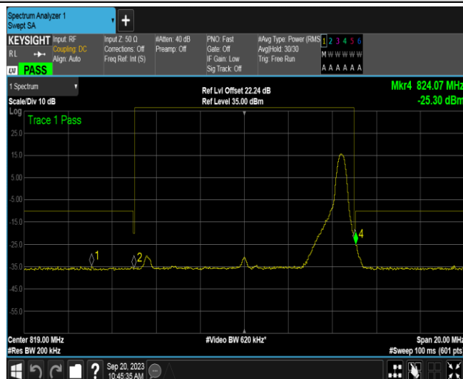
Band26B-10MHz-QPSK-26740-50RB#0
