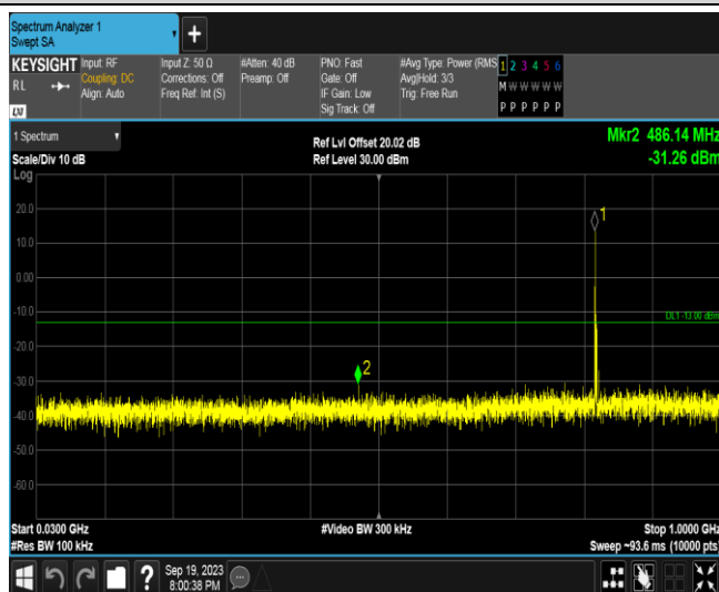
Band26B-3MHz-QPSK-26775-1RB#0-Range1:30~1000MHz
