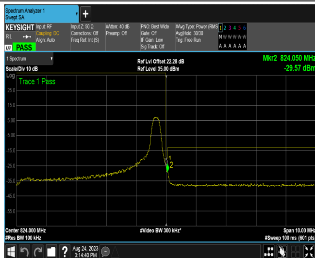
Band26B-5MHz-QPSK-26765-1RB#24
