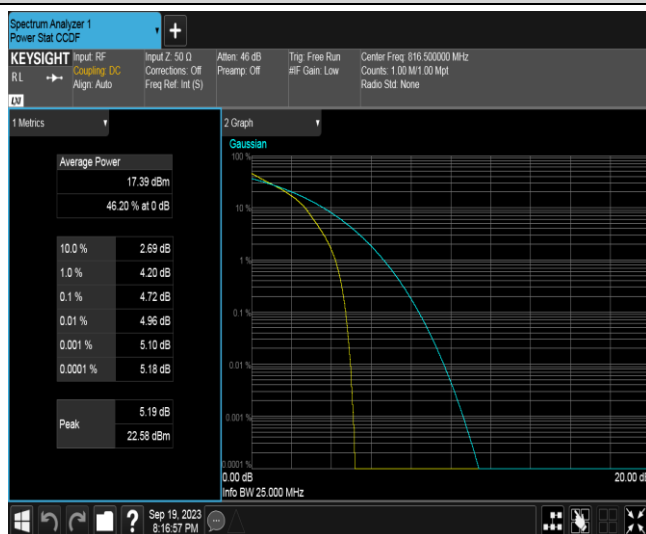
Band26B-5MHz-QPSK-26715-1RB#0
