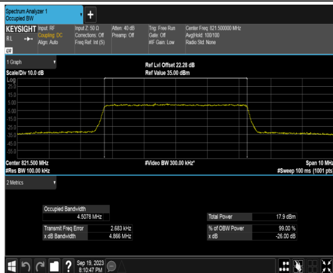
Band26B-5MHz-16QAM-26765-25RB#0
