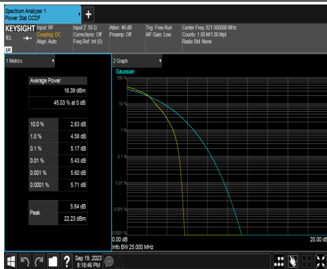
Band26B-5MHz-16QAM-26765-1RB#0
