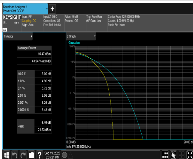
Band26B-3MHz-16QAM-26775-15RB#0
