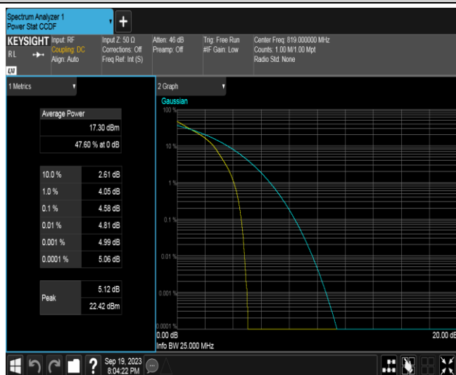
Band26B-3MHz-QPSK-26740-1RB#0
