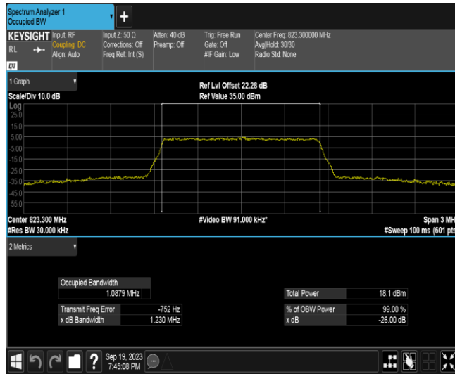
Band26B-3MHz-QPSK-26705-15RB#0
