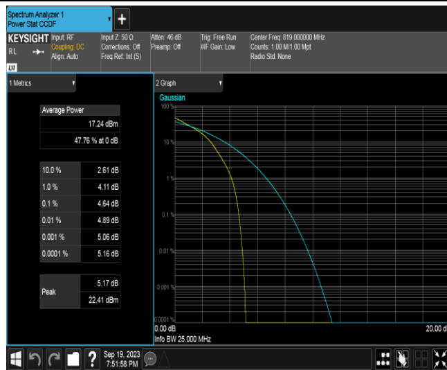
Band26B-1.4MHz-QPSK-26740-6RB#0
