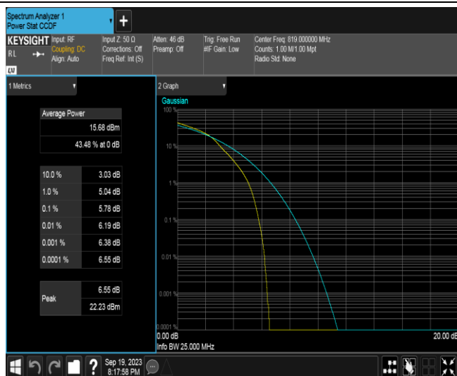
Band26B-5MHz-16QAM-26740-25RB#0
