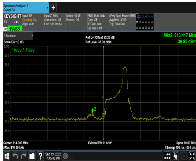
Band26B-1.4MHz-QPSK-26697-6RB#0
