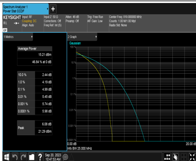
Band26B-10MHz-16QAM-26740-1RB#0
