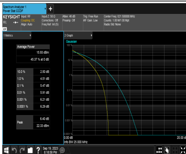
Band26B-5MHz-QPSK-26765-25RB#0
