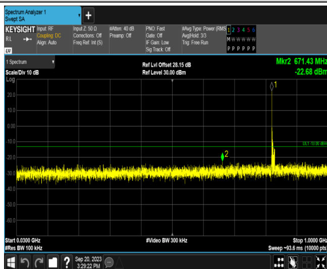
Band26A-10MHz-16QAM-26840-1RB#0-Range1:30~1000MHz
