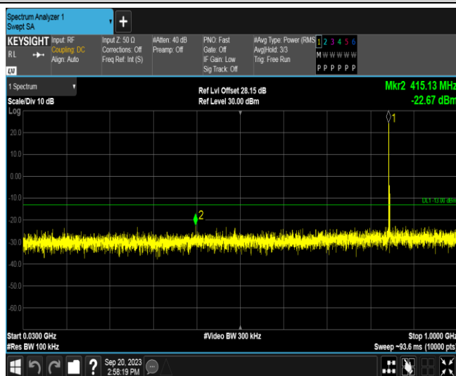
Band26A-3MHz-16QAM-27025-1RB#0-Range1:30~1000MHz
