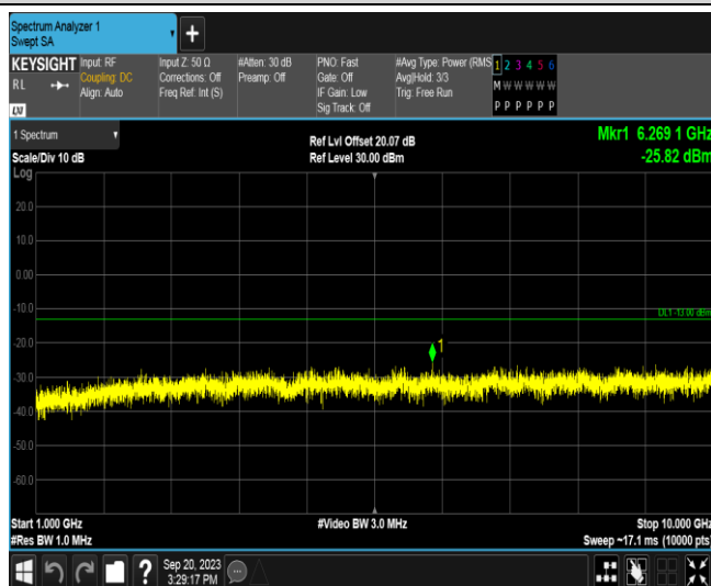
Band26A-10MHz-QPSK-26840-1RB#0-Range2:1000~10000MHz
