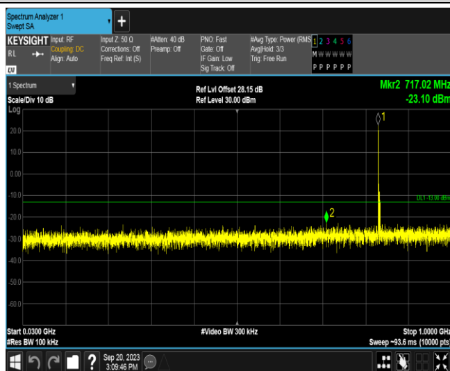
Band26A-5MHz-16QAM-26915-1RB#0-Range1:30~1000MHz
