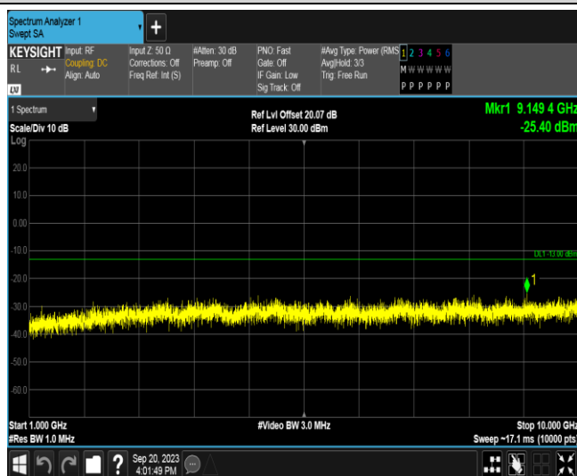
Band26A-15MHz-16QAM-26915-1RB#0-Range2:1000~10000MHz
