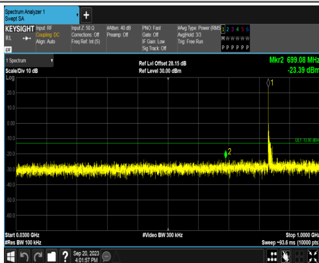
Band26A-15MHz-QPSK-26965-1RB#0-Range1:30~1000MHz
