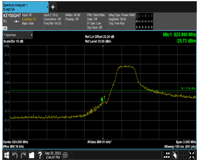
Band26A-1.4MHz-QPSK-26797-1RB#5
