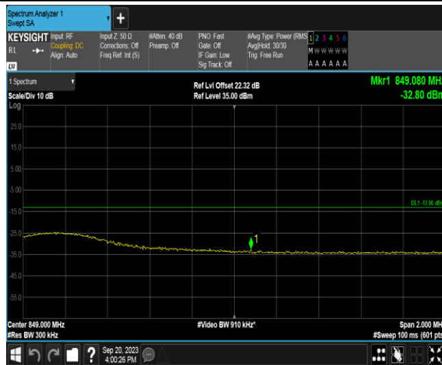
Band26A-15MHz-QPSK-26965-1RB#74
