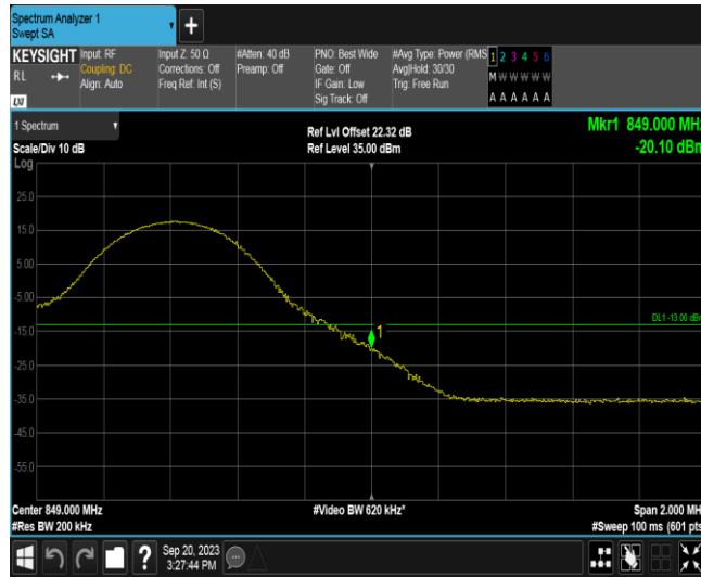
Band26A-10MHz-QPSK-26990-50RB#0
