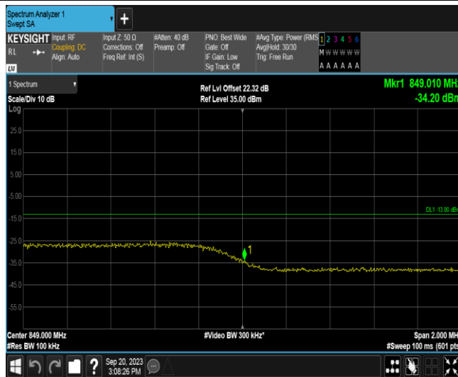
Band26A-5MHz-QPSK-27015-1RB#0
