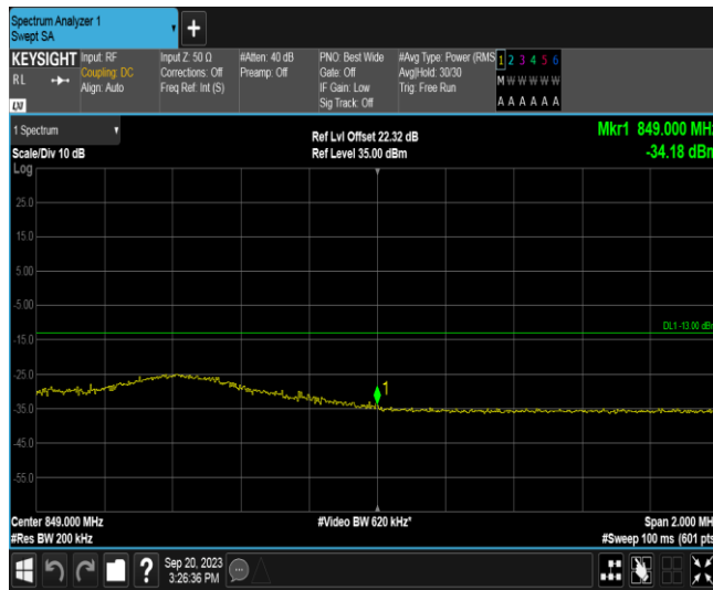
Band26A-10MHz-16QAM-26990-1RB#49
