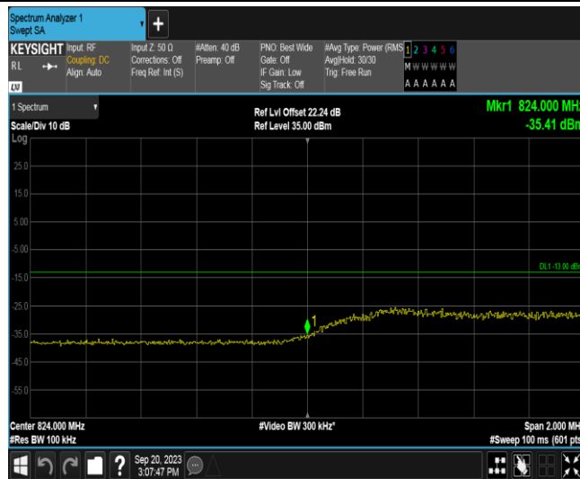
Band26A-5MHz-16QAM-26815-25RB#0
