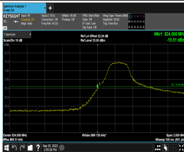
Band26A-3MHz-QPSK-26805-1RB#0
