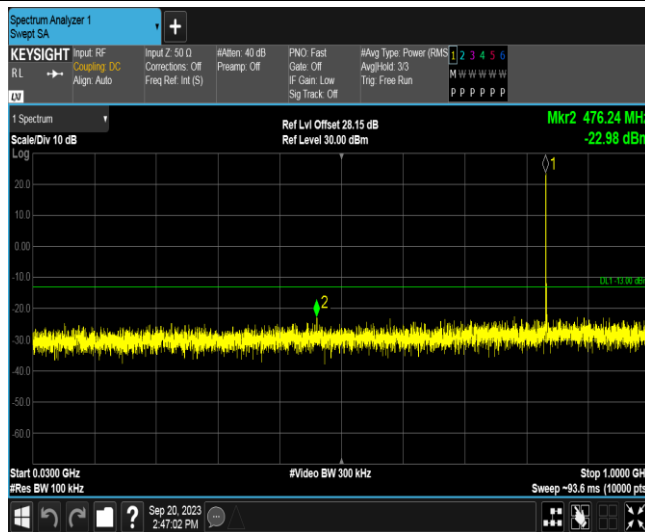
Band26A-1.4MHz-QPSK-26915-1RB#0-Range1:30~1000MHz
