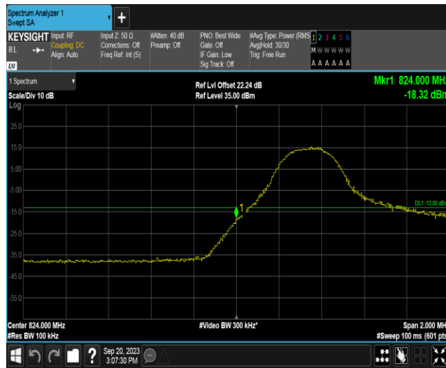
Band26A-5MHz-16QAM-26815-1RB#24
