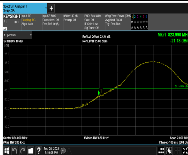
Band26A-10MHz-16QAM-26840-1RB#0
