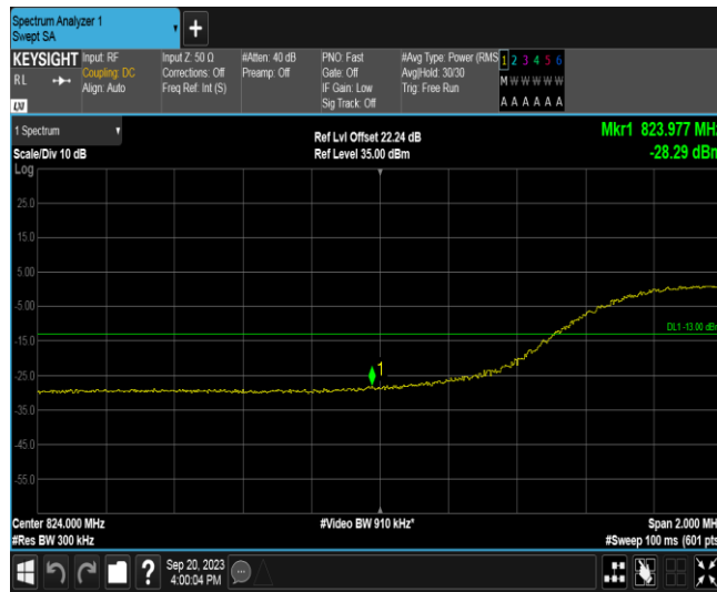
Band26A-15MHz-QPSK-26965-1RB#0
