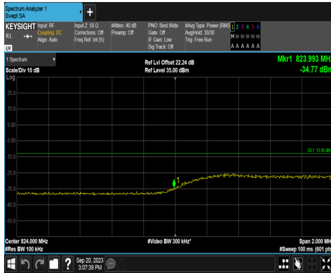
Band26A-5MHz-QPSK-26815-25RB#0
