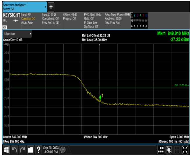
Band26A-10MHz-QPSK-26840-1RB#0
