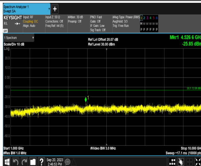
Band26A-1.4MHz-16QAM-26797-1RB#0-Range2:1000~10000MHz
