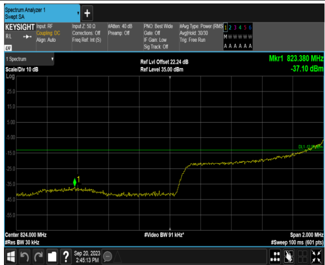
Band26A-1.4MHz-16QAM-26797-1RB#5
