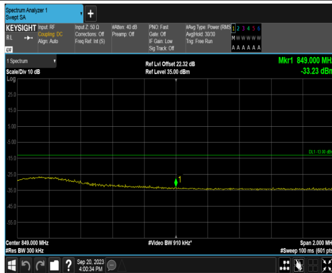
Band26A-15MHz-16QAM-26965-1RB#0
