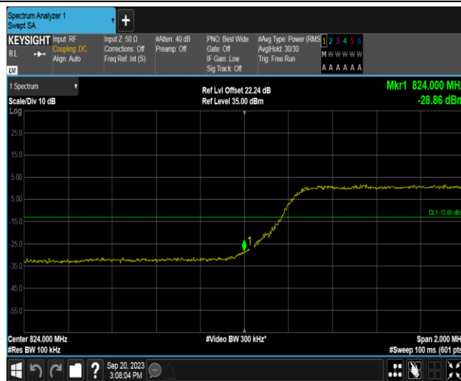
Band26A-5MHz-16QAM-26815-25RB#0
