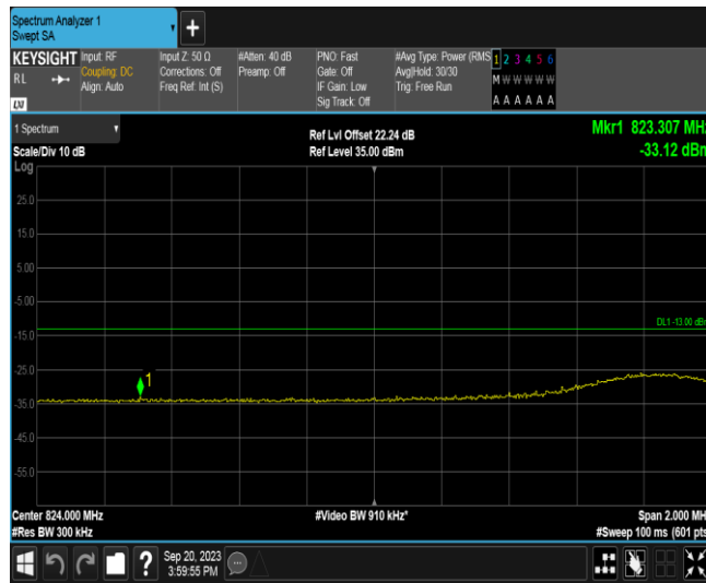
Band26A-15MHz-16QAM-26865-75RB#0
