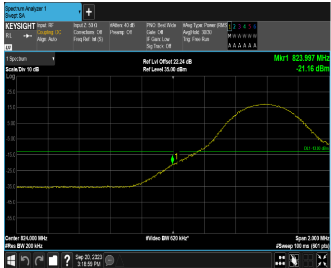
Band26A-10MHz-QPSK-26840-1RB#49
