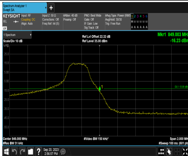
Band26A-3MHz-QPSK-27025-15RB#0
