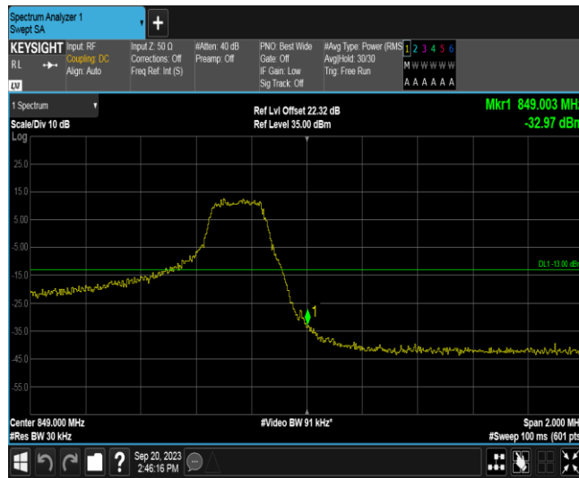
Band26A-1.4MHz-16QAM-27033-6RB#0
