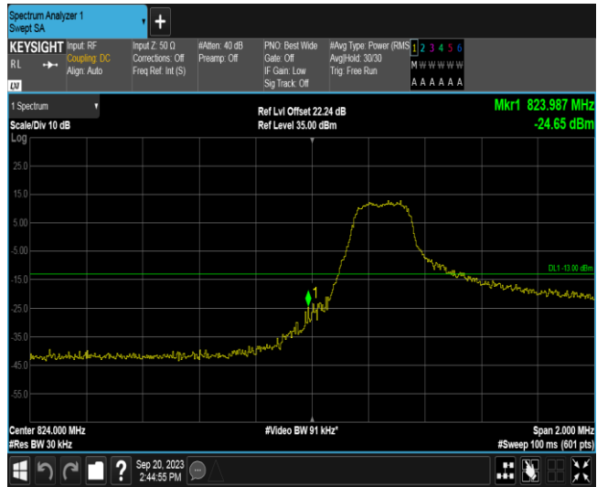
Band26A-1.4MHz-16QAM-26797-1RB#5
