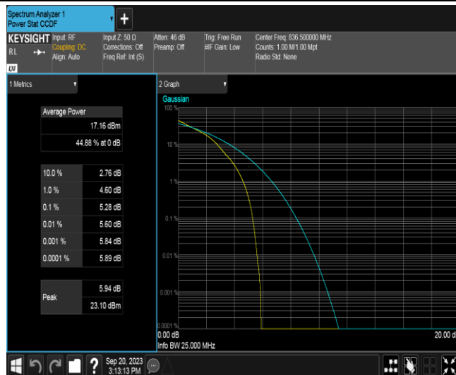
Band26A-5MHz-QPSK-26915-25RB#0
