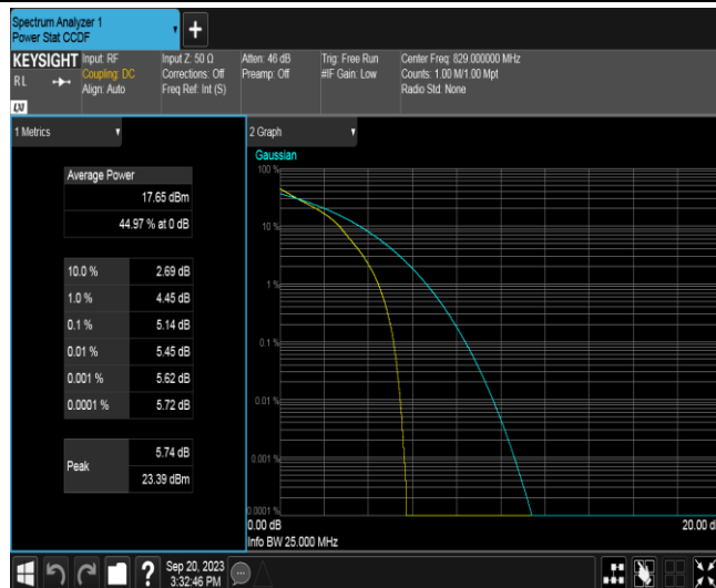
Band26A-10MHz-QPSK-26840-50RB#0
