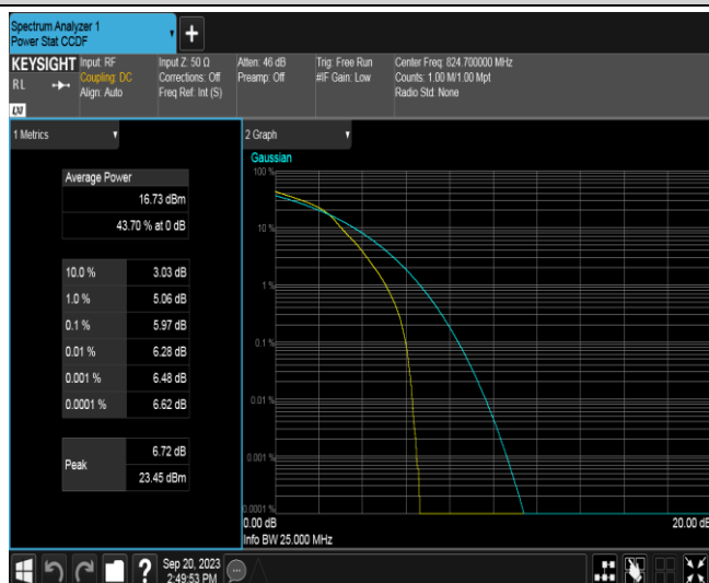
Band26A-1.4MHz-16QAM-26797-6RB#0
