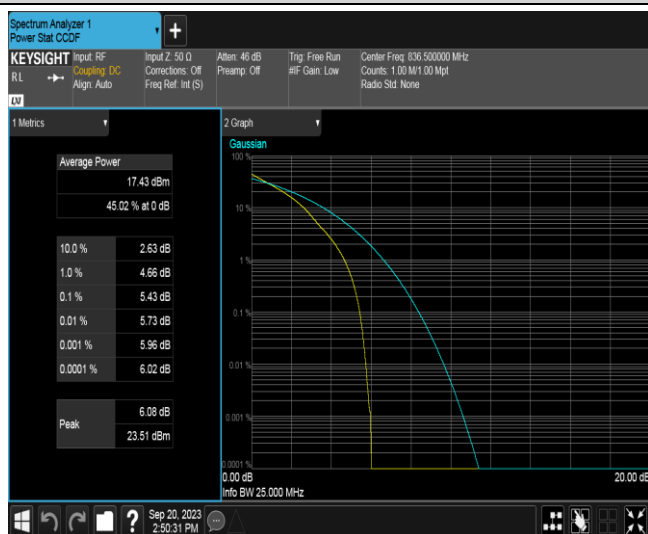
Band26A-1.4MHz-QPSK-26915-1RB#0
