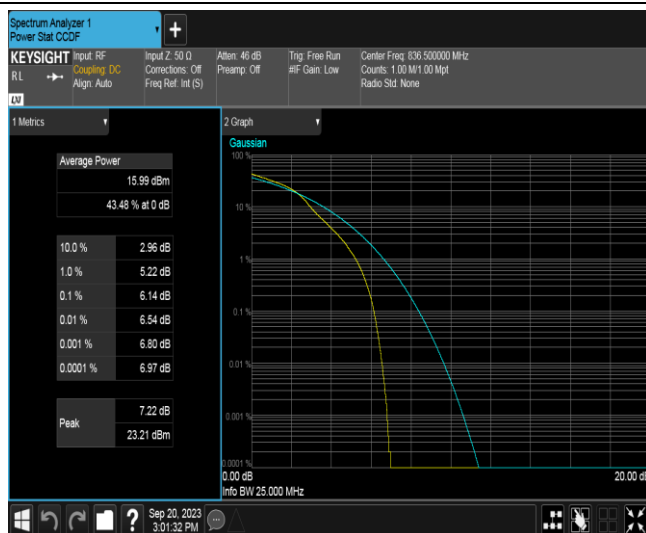
Band26A-3MHz-16QAM-26915-15RB#0
