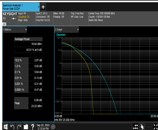
Band26A-5MHz-16QAM-26915-1RB#0
