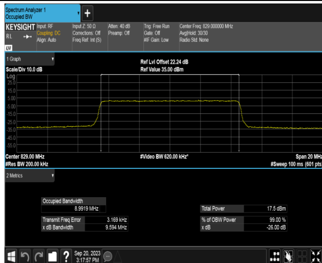
Band26A-10MHz-QPSK-26915-50RB#0
