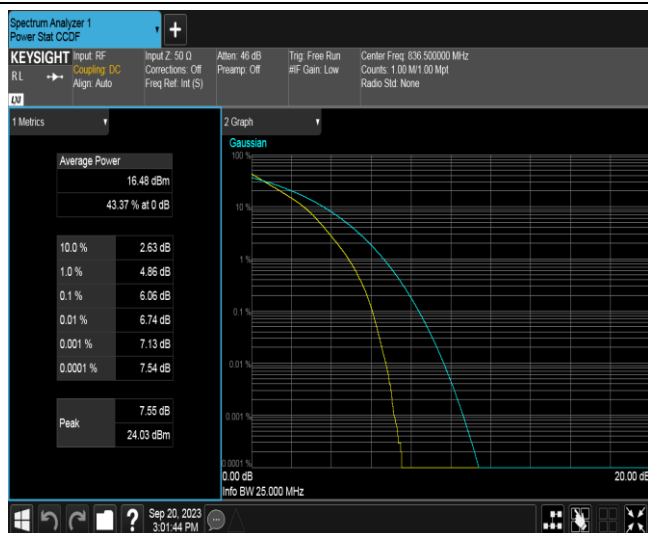
Band26A-3MHz-QPSK-27025-1RB#0
