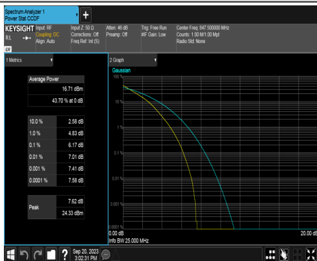
Band26A-3MHz-QPSK-27025-15RB#0
