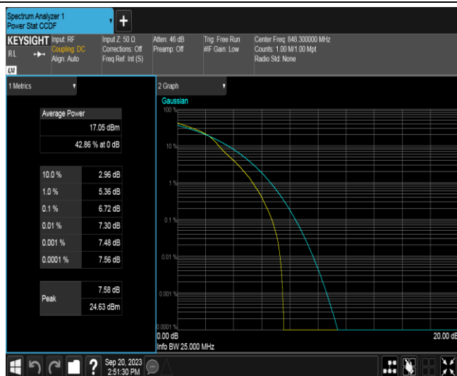
Band26A-1.4MHz-16QAM-27033-6RB#0
