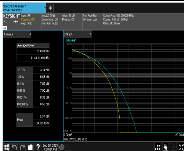
Band26A-15MHz-16QAM-26915-75RB#0
