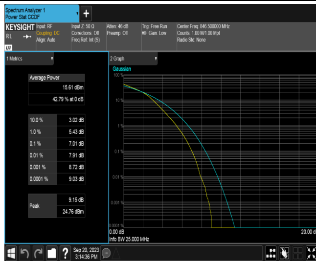
Band26A-10MHz-QPSK-26840-1RB#0
