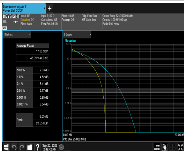
Band26A-1.4MHz-QPSK-26797-6RB#0
