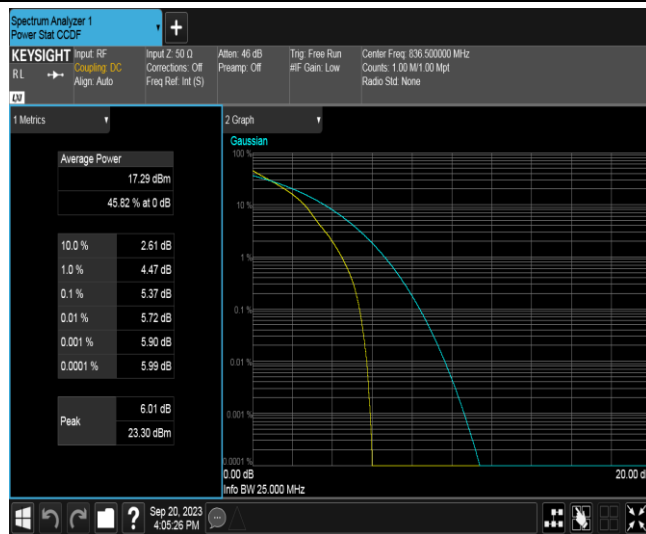
Band26A-15MHz-QPSK-26915-75RB#0
