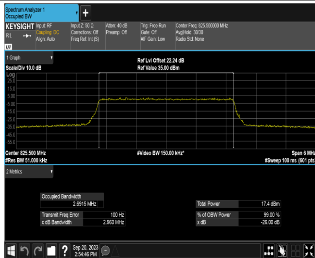
Band26A-3MHz-16QAM-26805-15RB#0
