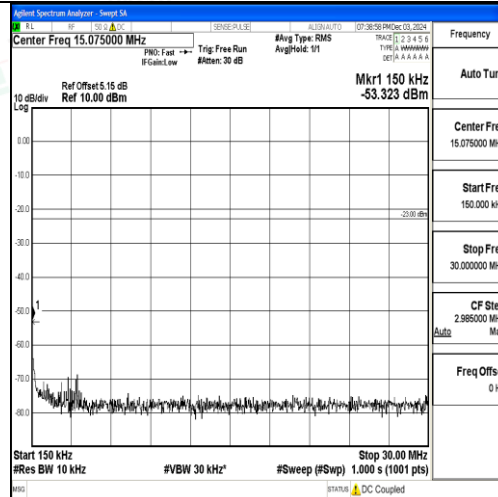
Band71_15MHz_16QAM_133397_1RB#0_0.15~30_0.15~30
