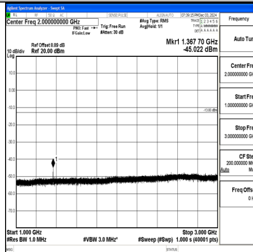
Band71_15MHz_16QAM_133397_1RB#0_1000~3000_1000~3000
