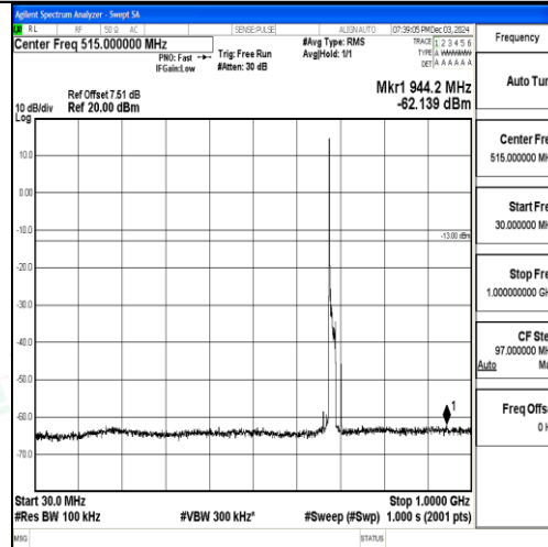
Band71_15MHz_16QAM_133397_1RB#0_30~1000_30~1000
