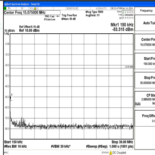
Band12_10MHz_QPSK_23095_1RB#0_0.15~30_0.15~30
