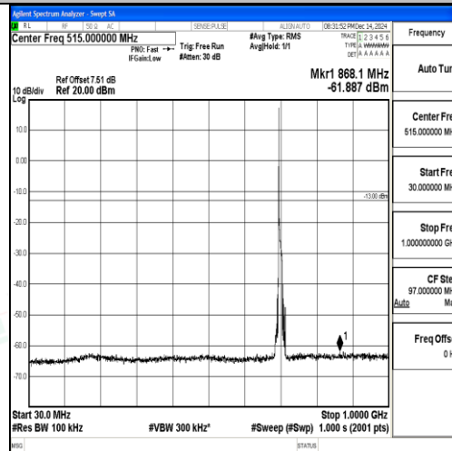
Band12_10MHz_QPSK_23095_1RB#0_30~1000_30~1000
