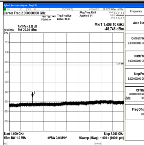
Band12_10MHz_QPSK_23095_1RB#0_1000~3000_1000~3000
