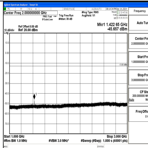
Band12_5MHz_16QAM_23155_1RB#0_1000~3000_1000~3000
