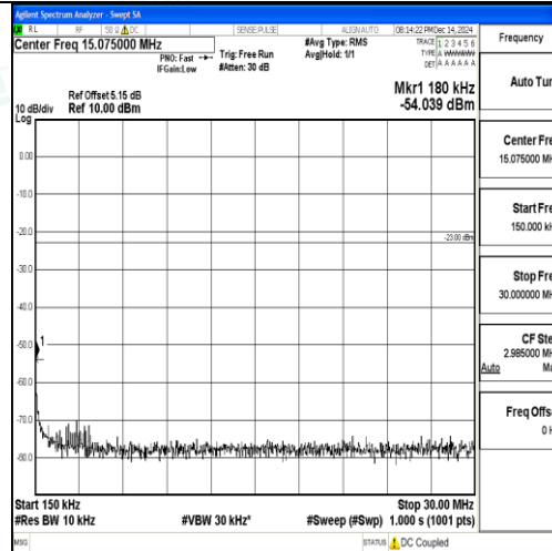
Band12_5MHz_16QAM_23155_1RB#0_0.15~30_0.15~30
