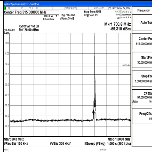
Band12_5MHz_16QAM_23155_1RB#0_30~1000_30~1000
