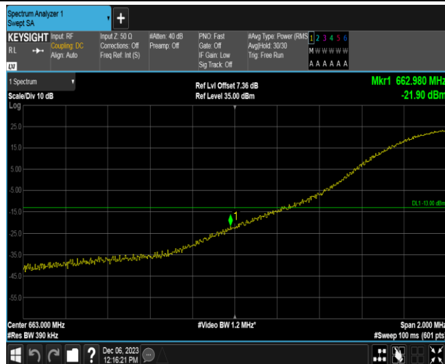
Band71-20MHz-16QAM-133222-1RB#99
