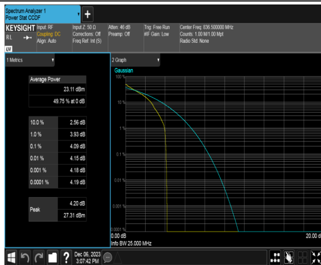
Band26-3MHz-QPSK-26915-1RB#0
