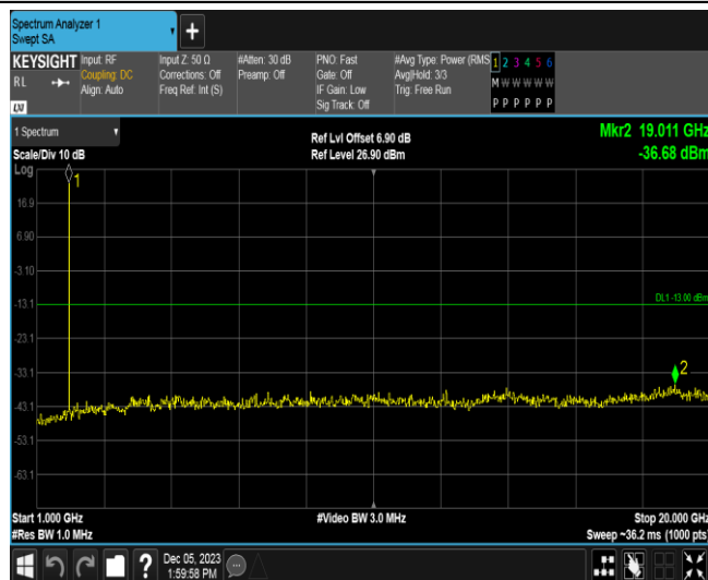
Band25-5MHz-QPSK-26665-1RB#0-Range2:1000~20000MHz
