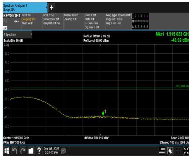
Band25-15MHz-16QAM-26615-1RB#74
