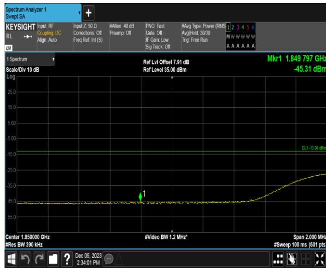
Band25-20MHz-16QAM-26140-100RB#0
