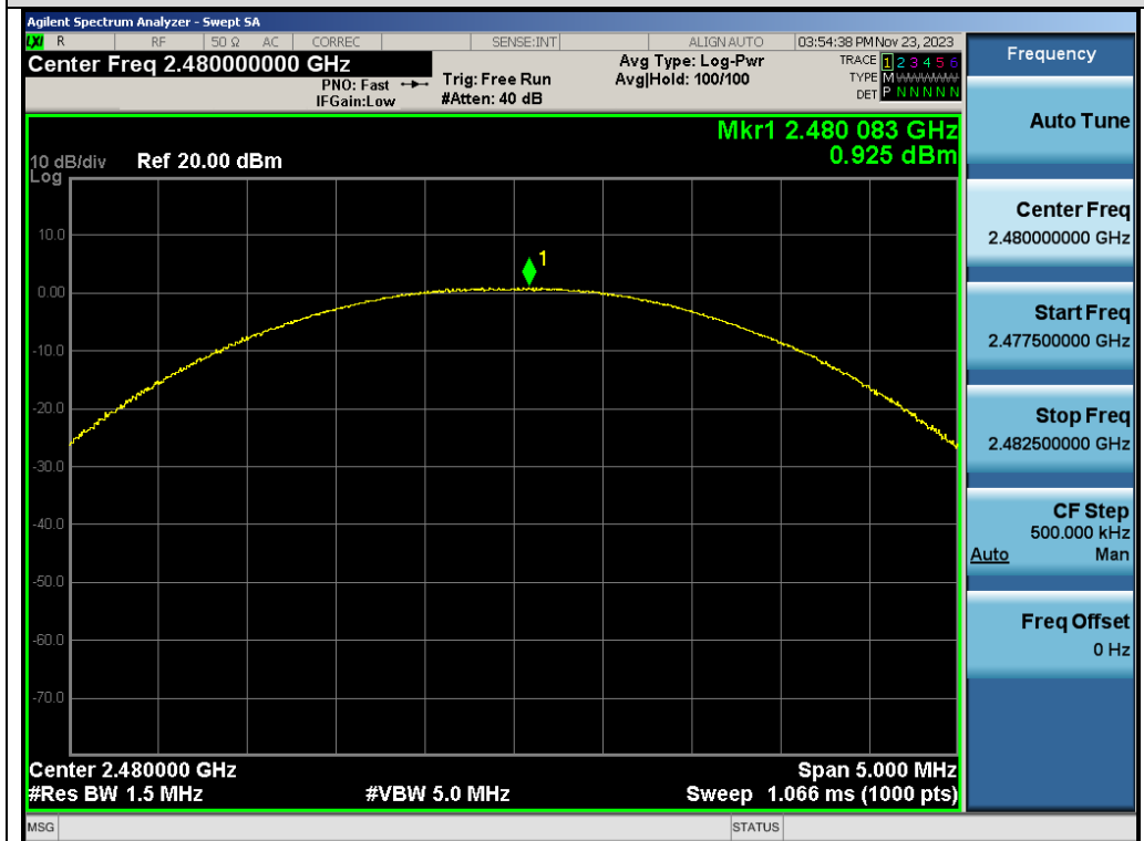
Test_Graph_EDR_ANT1_2480_2Mbps_Peak Power
