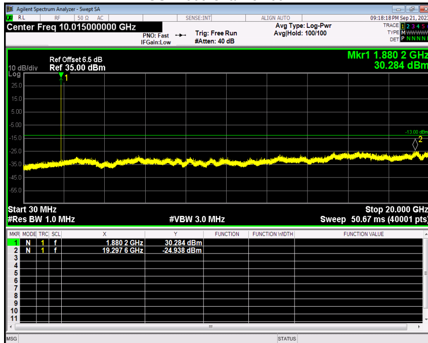
GSM1900 Channel=661
