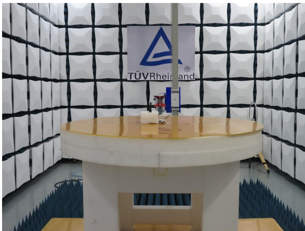
Photograph 4: Set-up photo for Radiated Spurious Emission, above 1 GHz (Ant 2#)
