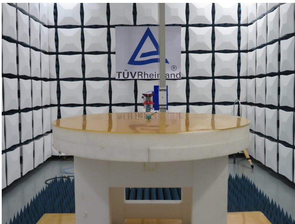
Photograph 2: Set-up photo for Radiated Spurious Emission, above 1 GHz (Ant 1#)
