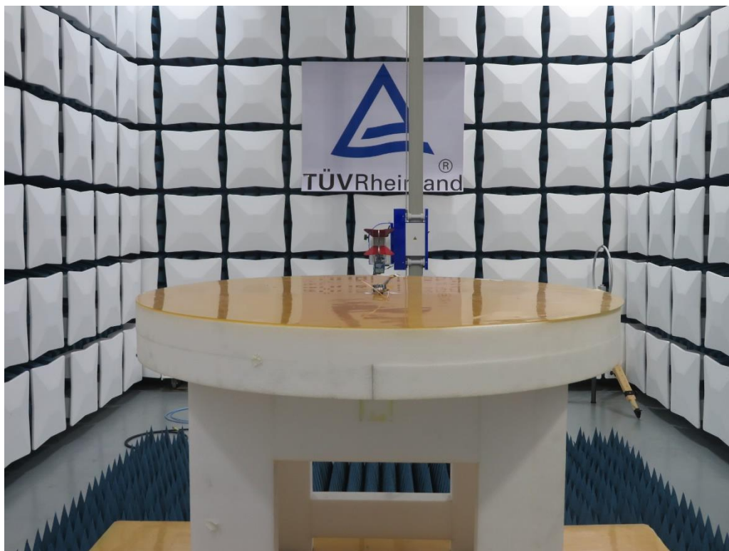
Photograph 6: Set-up photo for Radiated Spurious Emission, above 1 GHz(Ant 3#)
