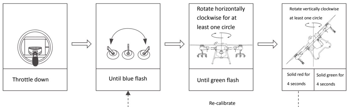
Figure 1-4-7 Compass Calibration
