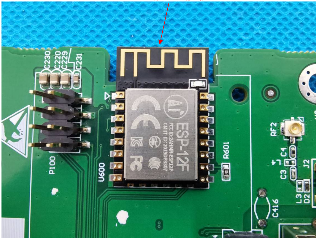
Wi-Fi Antenna
