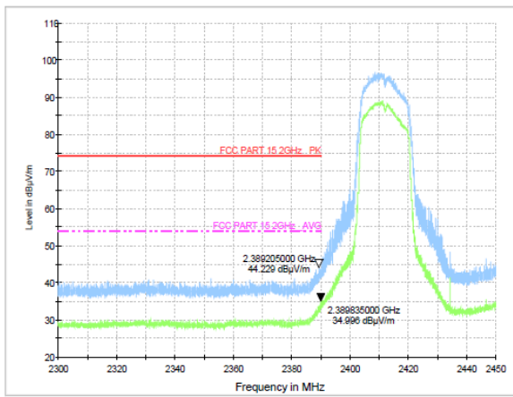
Test Mode: IEEE 802.11g-Low
