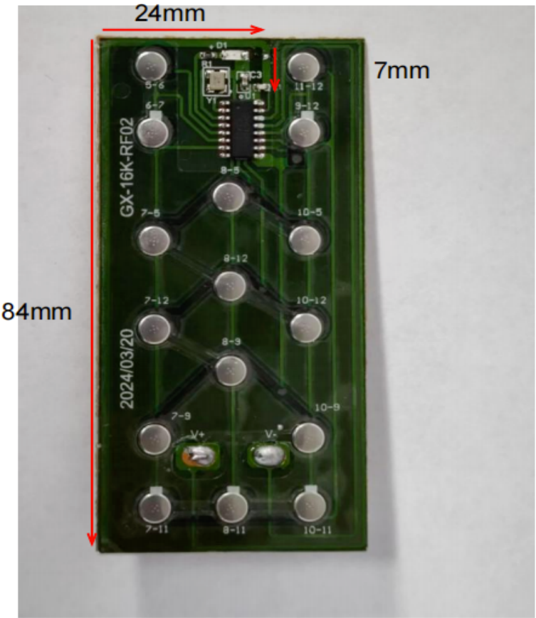
Antenna Photo &Length (mm)
