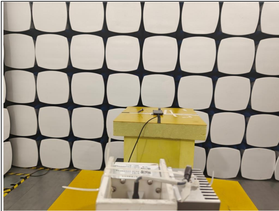
Radiated Spurious Emission: 18GHz-26.5GHz
